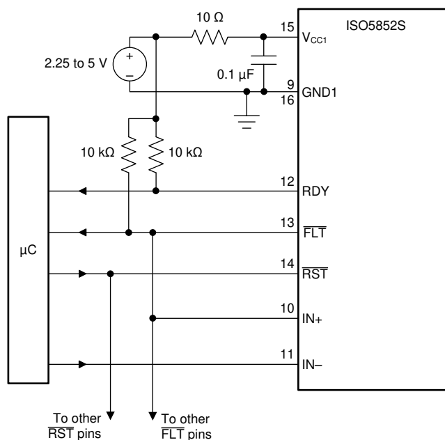
Figure 10-6. Global Shutdown With Inverting Input Configuration
