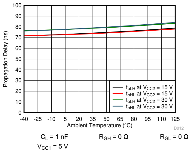
C_L = 1\text{ nF} R_{GH} = 0\ \Omega R_{GL} = 0\ \Omega V_{CC1} = 5\text{ V} Figure 7-25. Propagation Delay vs Temperature
