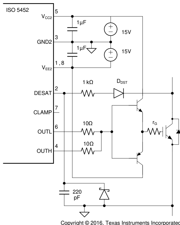
Figure 10-10. Current Buffer for Increased Drive Current
