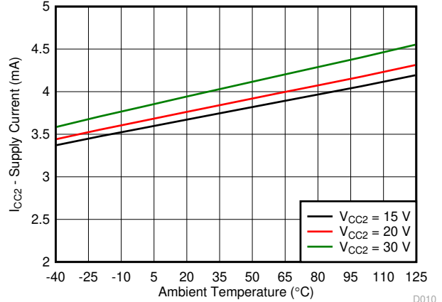
Input frequency = 1 kHz Figure 7-22. I_{CC2} Supply Current vs Temperature
