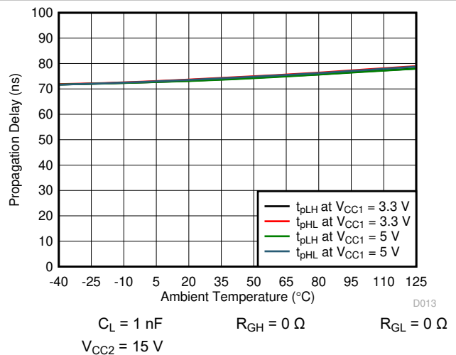
C_L = 1\text{ nF} R_{GH} = 0\ \Omega R_{GL} = 0\ \Omega V_{CC2} = 15\text{ V} Figure 7-26. Propagation Delay vs Temperature
