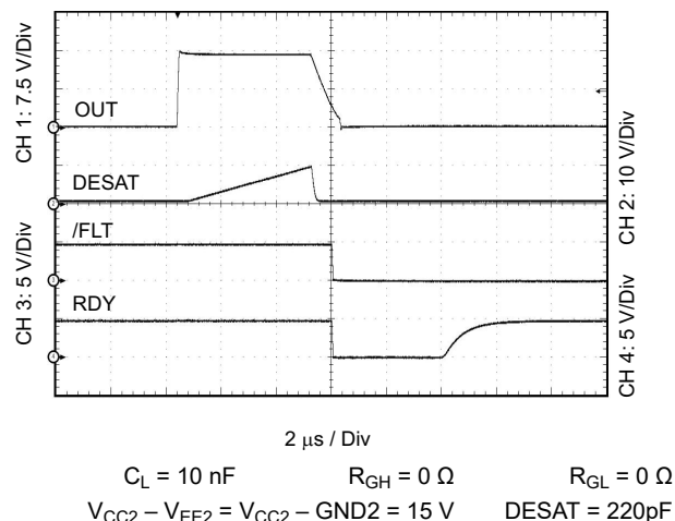
Figure 7-16. Output Transient Waveform DESAT, RDY and FLT
