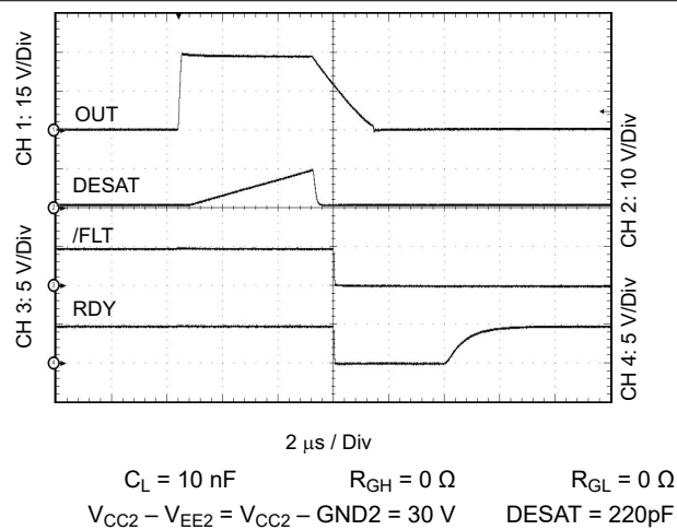
Figure 7-18. Output Transient Waveform DESAT, RDY and FLT
