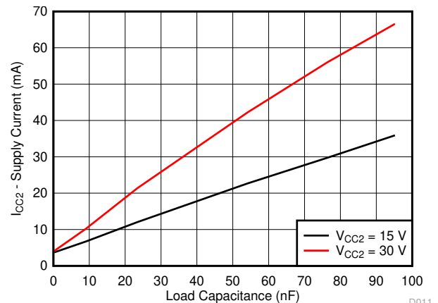
R_{GH} = 10\ \Omega R_{GL} = 5\ \Omega , 20 kHz Figure 7-24. I_{CC2} Supply Current vs Load Capacitance
