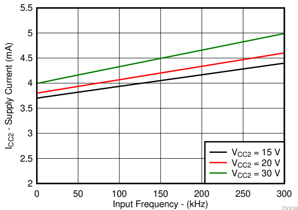
No C_L Figure 7-23. I_{CC2} Supply Current vs Input Frequency
