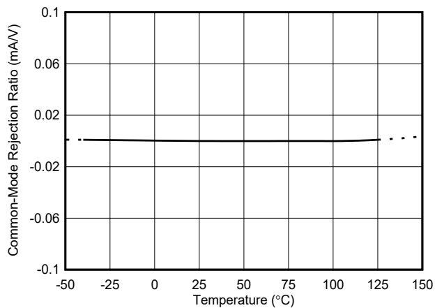
Figure 5-5. Current Common-Mode Rejection Ratio vs Temperature
