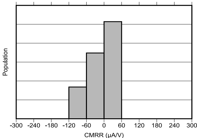
Figure 5-4. Common-Mode Rejection Ratio Production Distribution
