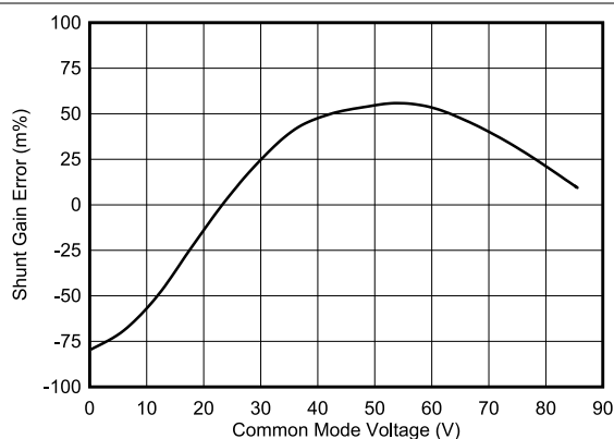
Figure 5-8. Current Gain Error vs Common-Mode Voltage
