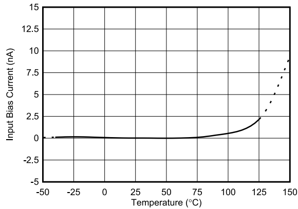
Figure 5-14. Input Bias Current vs Temperature
