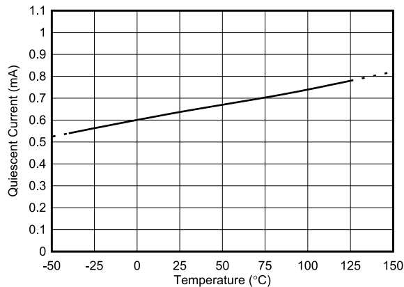
Figure 5-16. Active I_Q vs Temperature
