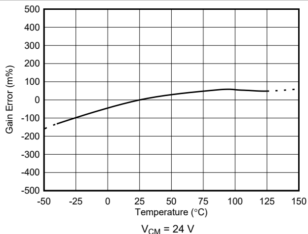
Figure 5-7. Current Gain Error vs Temperature
