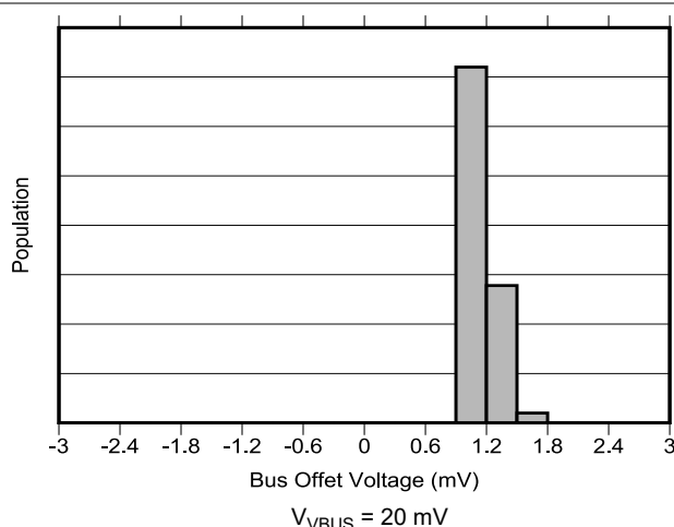
Figure 5-9. Bus Input Offset Voltage Production Distribution
