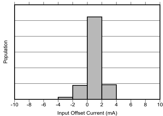
Figure 5-2. Shunt Input Offset Current Production Distribution
