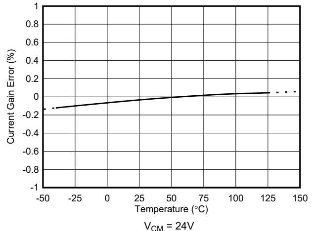
Figure 5-7. Current Gain Error vs Temperature
