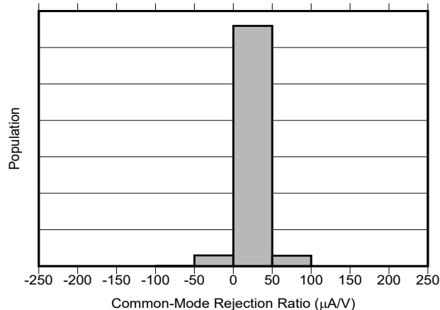
Figure 5-4. Common-Mode Rejection Ratio Production Distribution
