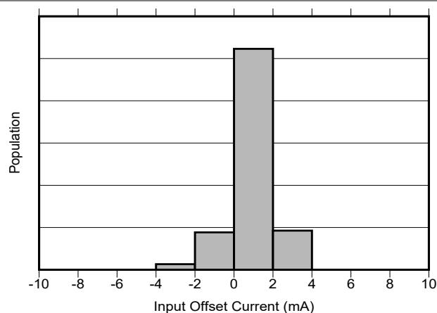
Figure 5-2. Shunt Input Offset Current Production Distribution
