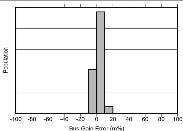
Figure 5-11. Bus Input Gain Error Production Distribution
