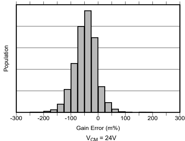
Figure 5-6. Current Gain Error Production Distribution
