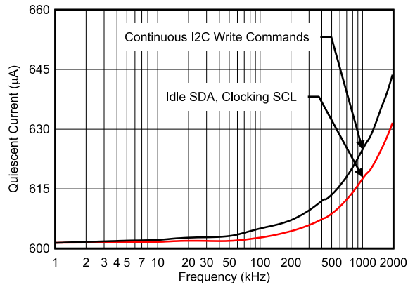
Figure 5-20. Active I_Q vs Clock Frequency
