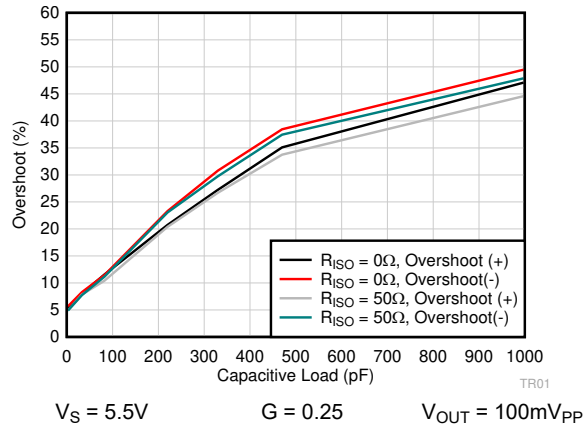
Figure 6-63. Small-Signal Overshoot vs Capacitive Load
