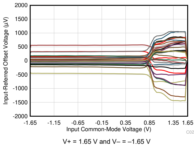
Figure 7-17. Input Referred Offset Voltage vs Input Common-Mode Voltage
