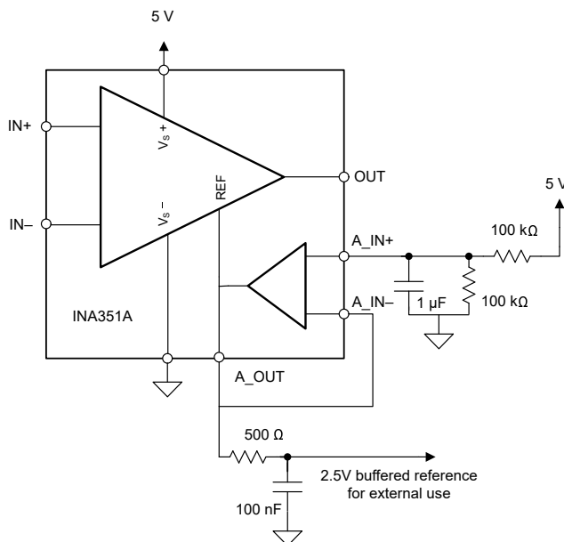
Figure 9-1. INA351A in Reference Buffer Configuration
