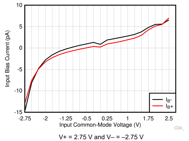
Figure 7-18. Input Bias Current vs Input Common-Mode Voltage
