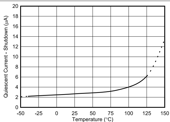
Figure 5-21. Shutdown I_Q vs Temperature
