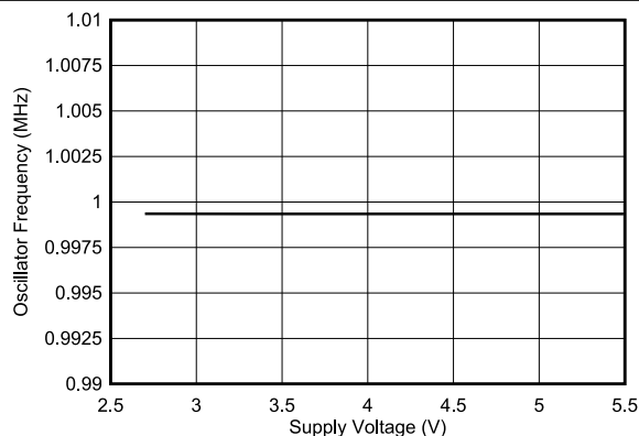
Figure 5-24. Internal Clock Frequency vs Power Supply
