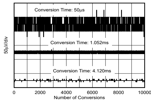
Figure 6-4. Noise vs. Conversion Time (Averaging = 1)
