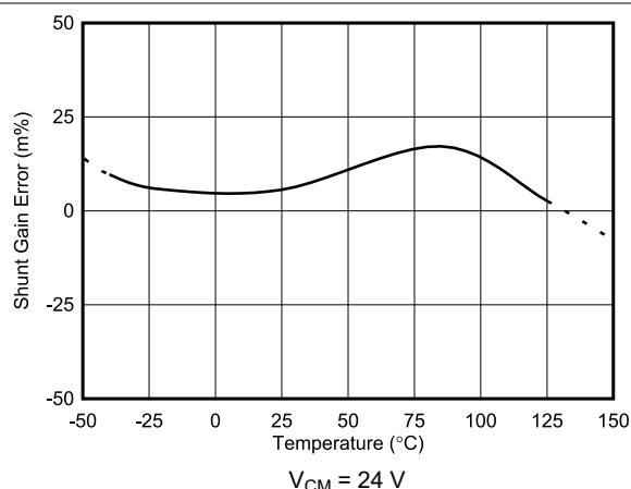
Figure 5-8. Shunt Input Gain Error vs Temperature
