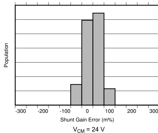
Figure 5-7. Shunt Input Gain Error Production Distribution
