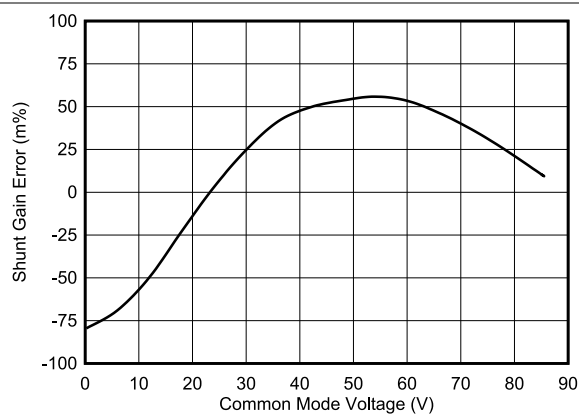
Figure 5-9. Shunt Input Gain Error vs Common-Mode Voltage
