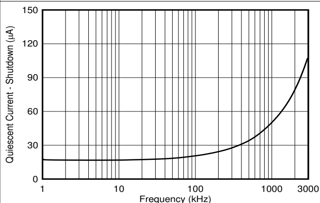
Figure 5-23. Shutdown I_Q vs Clock Frequency
