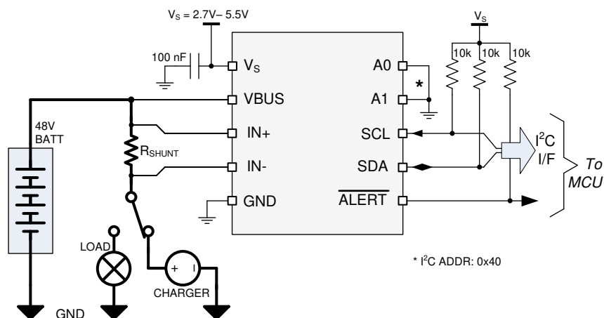
Figure 7-2. INA237-Q1 High-Side Sensing Application Diagram
