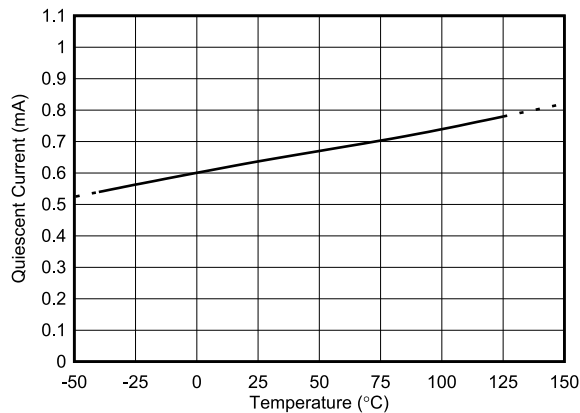
Figure 5-18. Active I_Q vs Temperature
