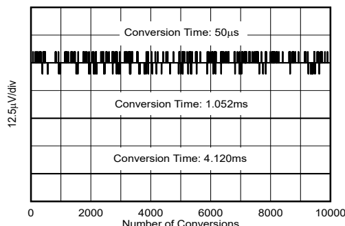
Figure 6-5. Noise vs. Conversion Time (Averaging = 128)
