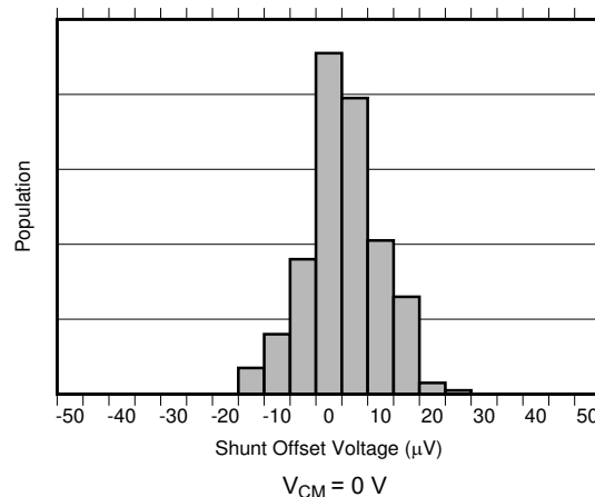
Figure 5-3. Shunt Input Offset Voltage Production Distribution
