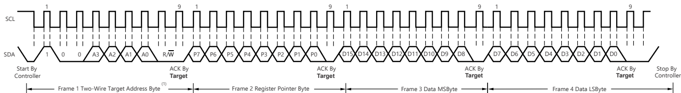
Figure 6-4. Timing Diagram for Write Word Format
