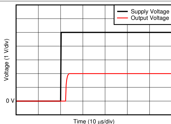
Figure 7-35. Start-Up Response
