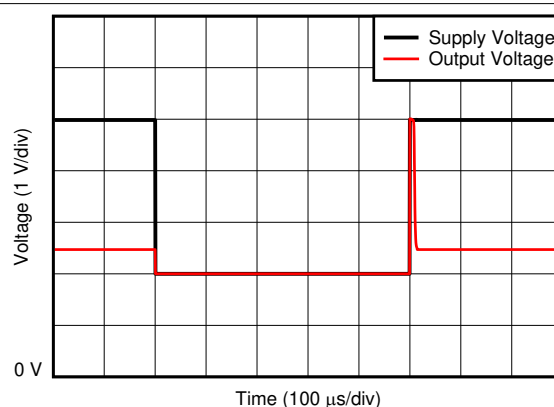
Figure 7-36. Brownout Recovery
