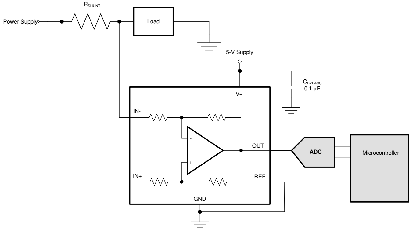
Figure 6-1. Typical Application
