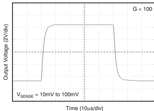
Figure 19. Step Response
