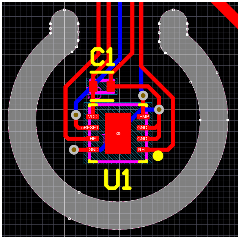
Figure 8-5. Layout Example
