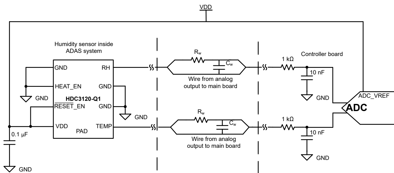
Figure 8-1. HDC3120-Q1 Connection to ADC
