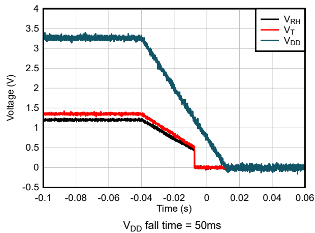
Figure 6-16. Power-down Response
