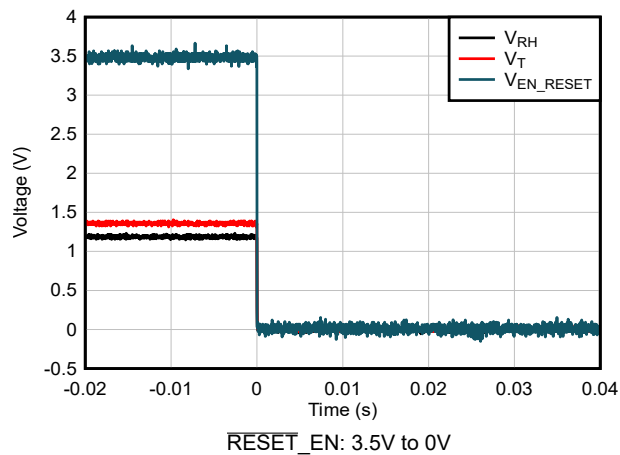
Figure 6-18. Disable Response
