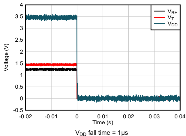
Figure 6-14. Power-down Response
