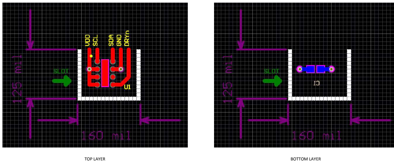
Figure 19. HDC1008 Layout
