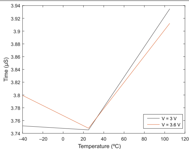
Figure 8-4. Intra-Pair Skew Ports C to A (μs)
