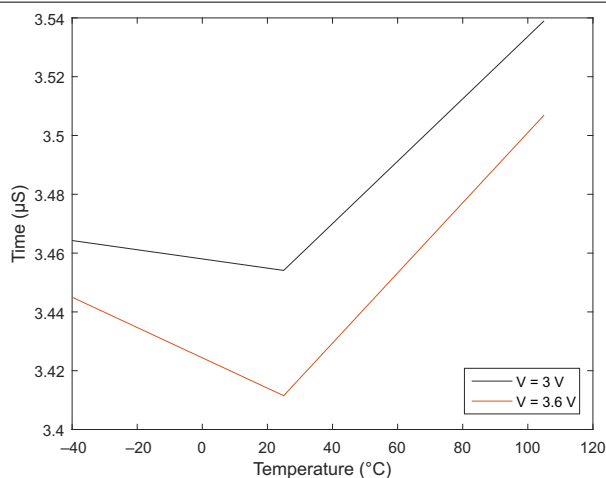
Figure 8-5. Intra-Pair Skew Ports C to B (μs)
