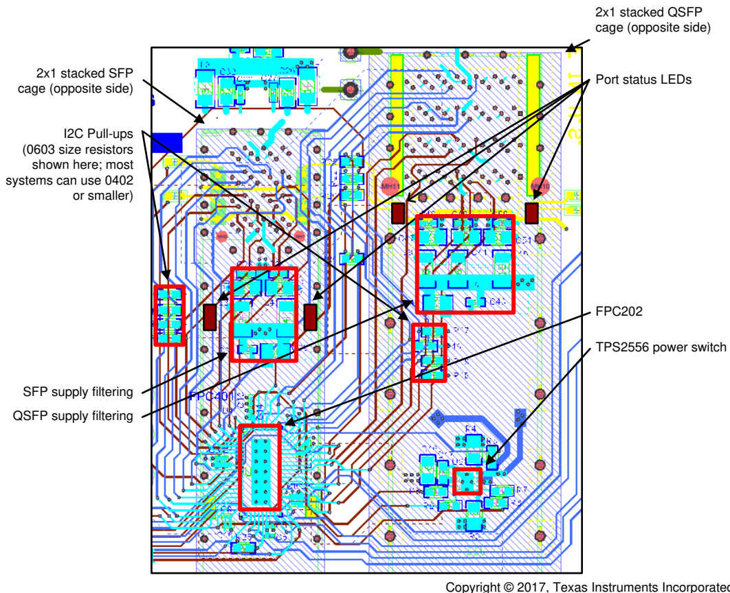
Figure 8-8. Layout Example
