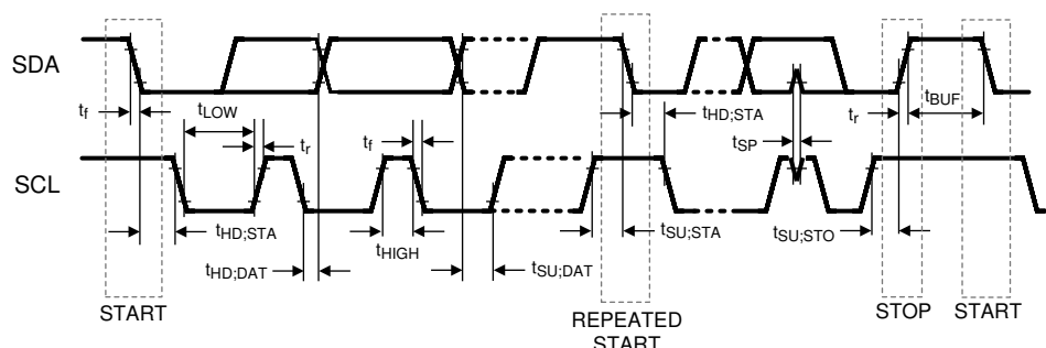
Figure 6-1. I 2 C Timing
