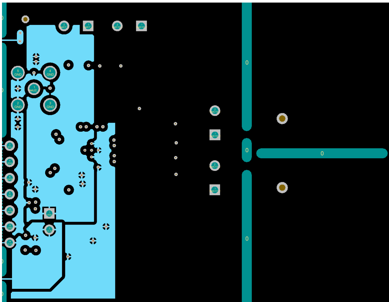
Figure 8-12. Example PCB Layout: Mid-Layer 2 (Power)
