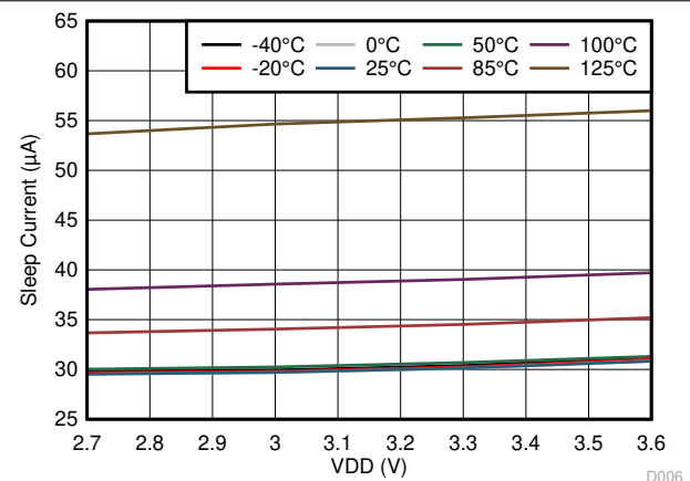
Figure 6-5. Sleep Mode IDD vs VDD
