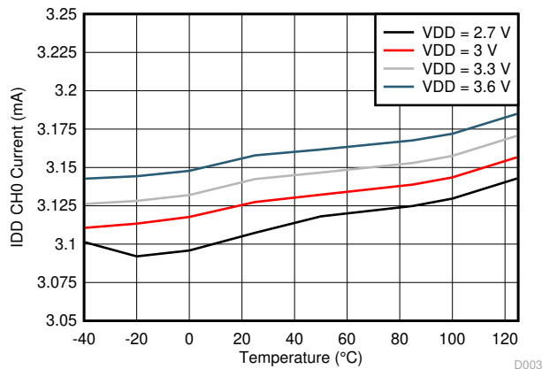
Figure 6-2. Active Mode IDD vs Temperature
