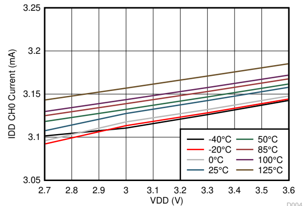
Figure 6-3. Active Mode IDD vs VDD
