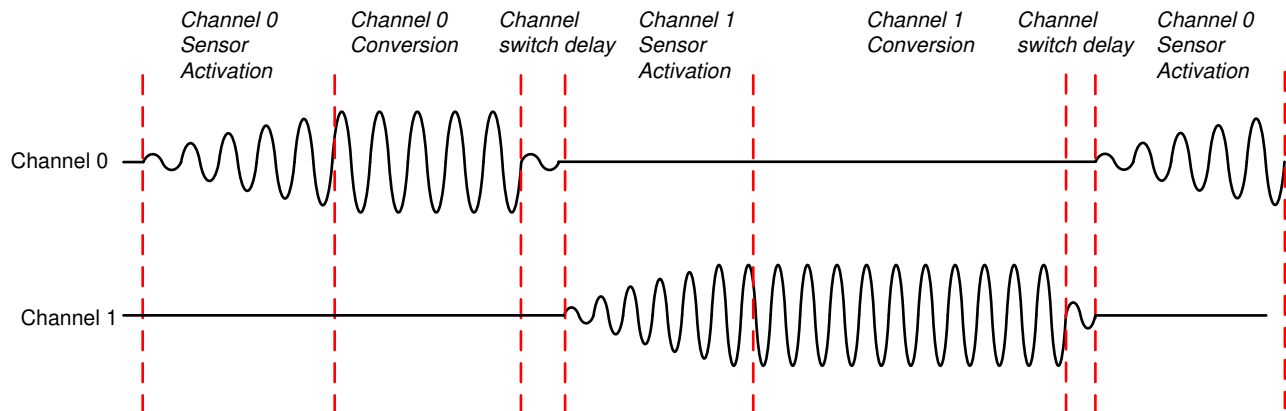
Figure 7-4. Multi-Channel Mode Sequencing
