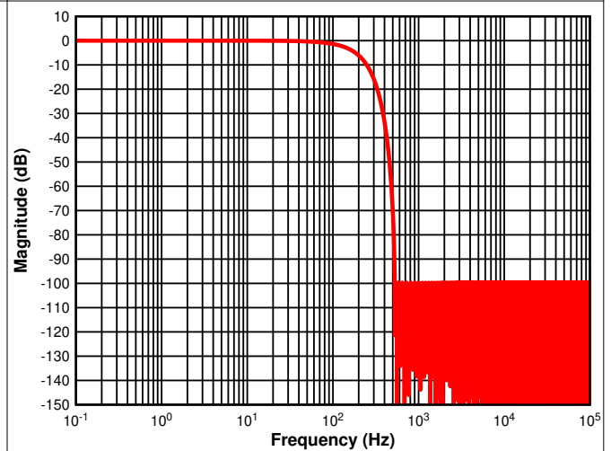
Figure 5-7. Frequency Response 100S/s
