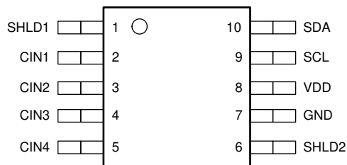
Figure 4-1. DGS Package 10 Pin VSSOP Top View
