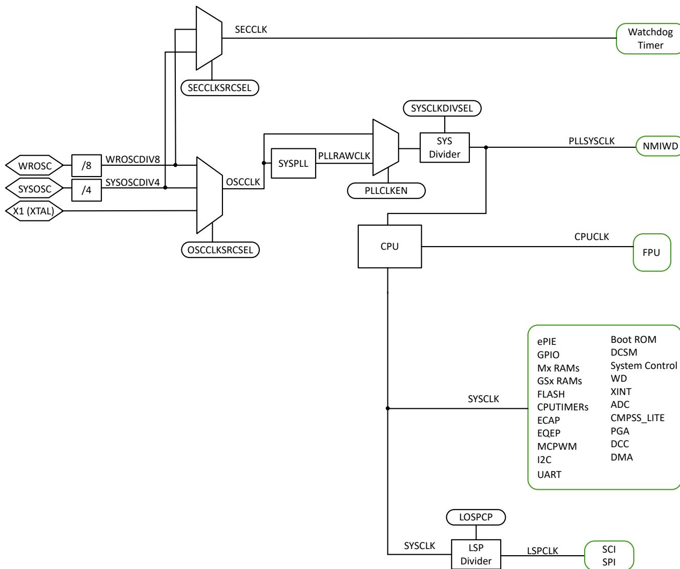
Figure 6-8. Clocking System
