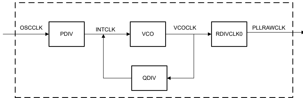
Figure 6-9. System PLL
