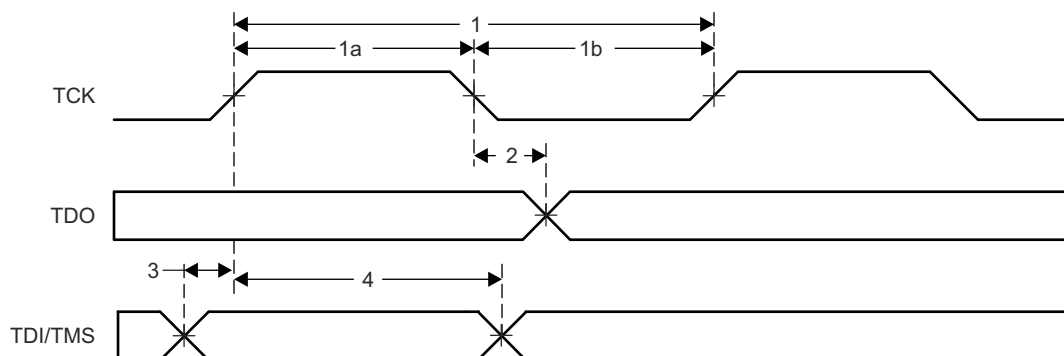
Figure 6-21. JTAG Timing
