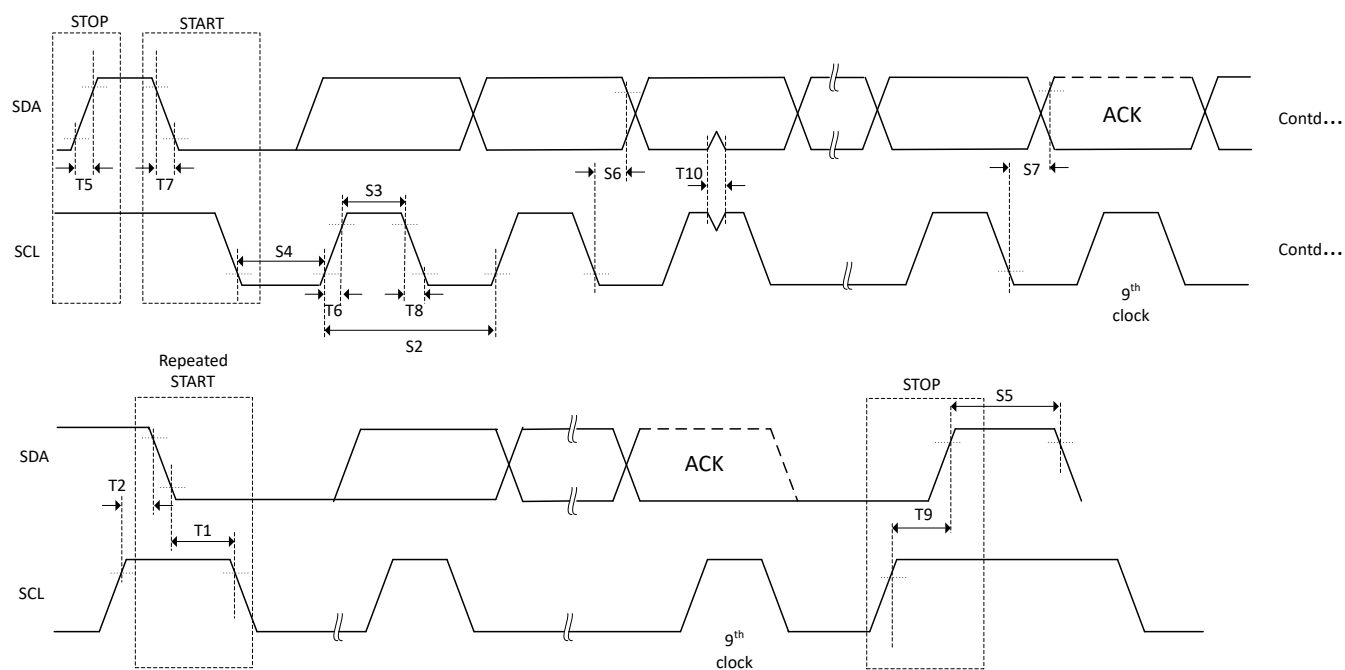
Figure 6-55. I2C Timing Diagram
