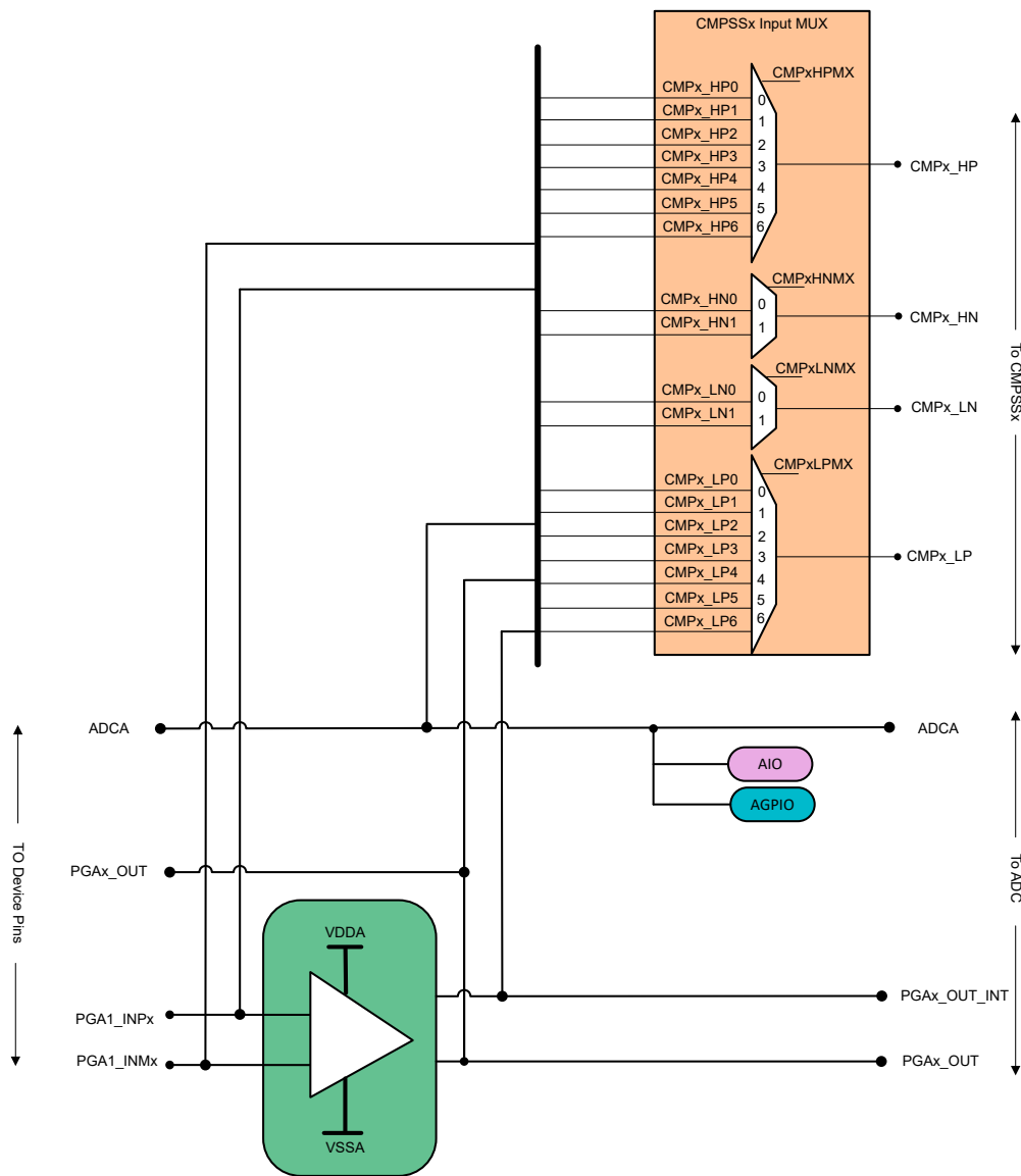
Figure 6-32. Analog Group Connections
