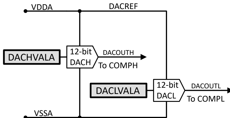
Figure 6-40. Reference DAC Block Diagram
