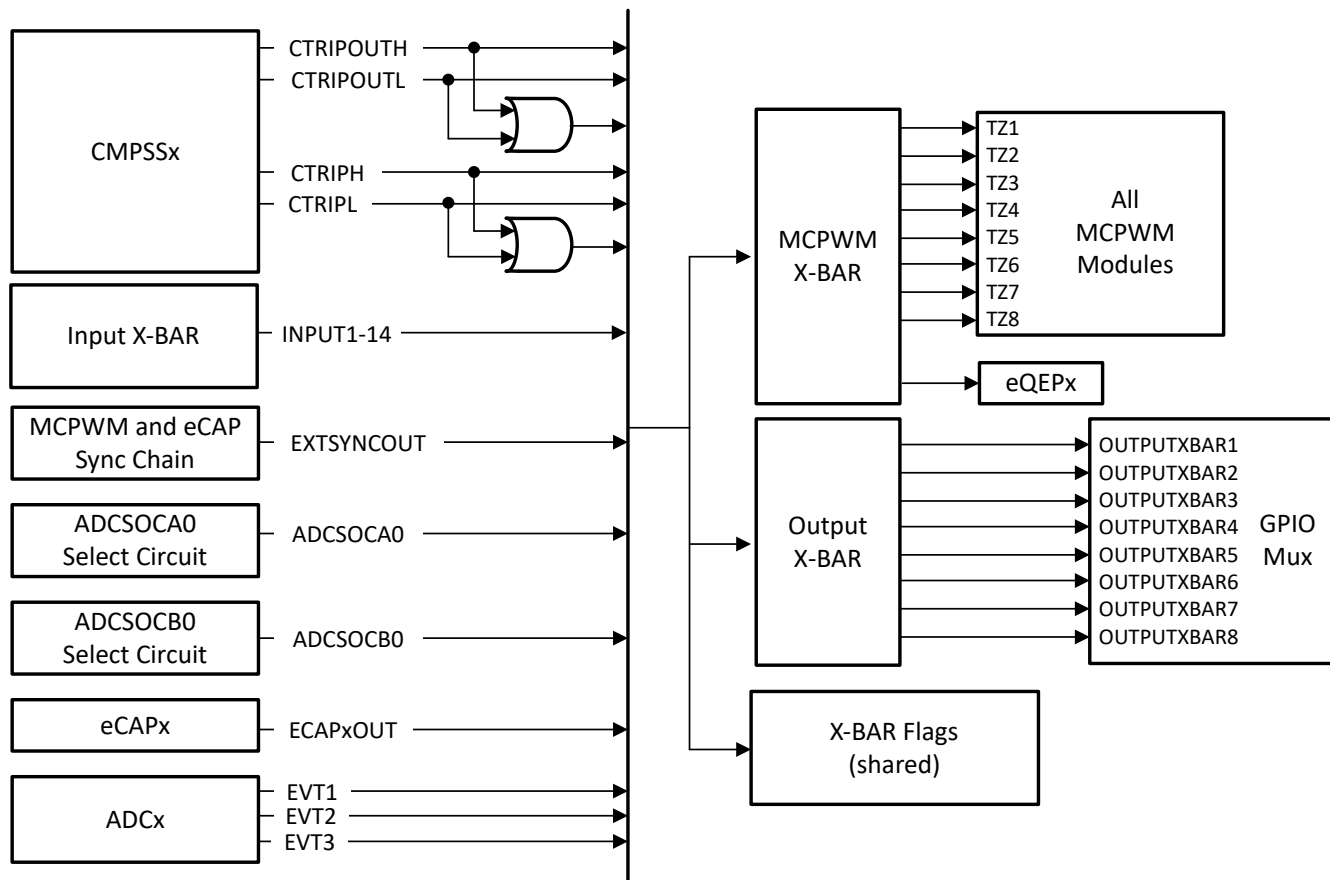
Figure 5-5. GPIO Output X-BAR and PWM X-BAR Sources
