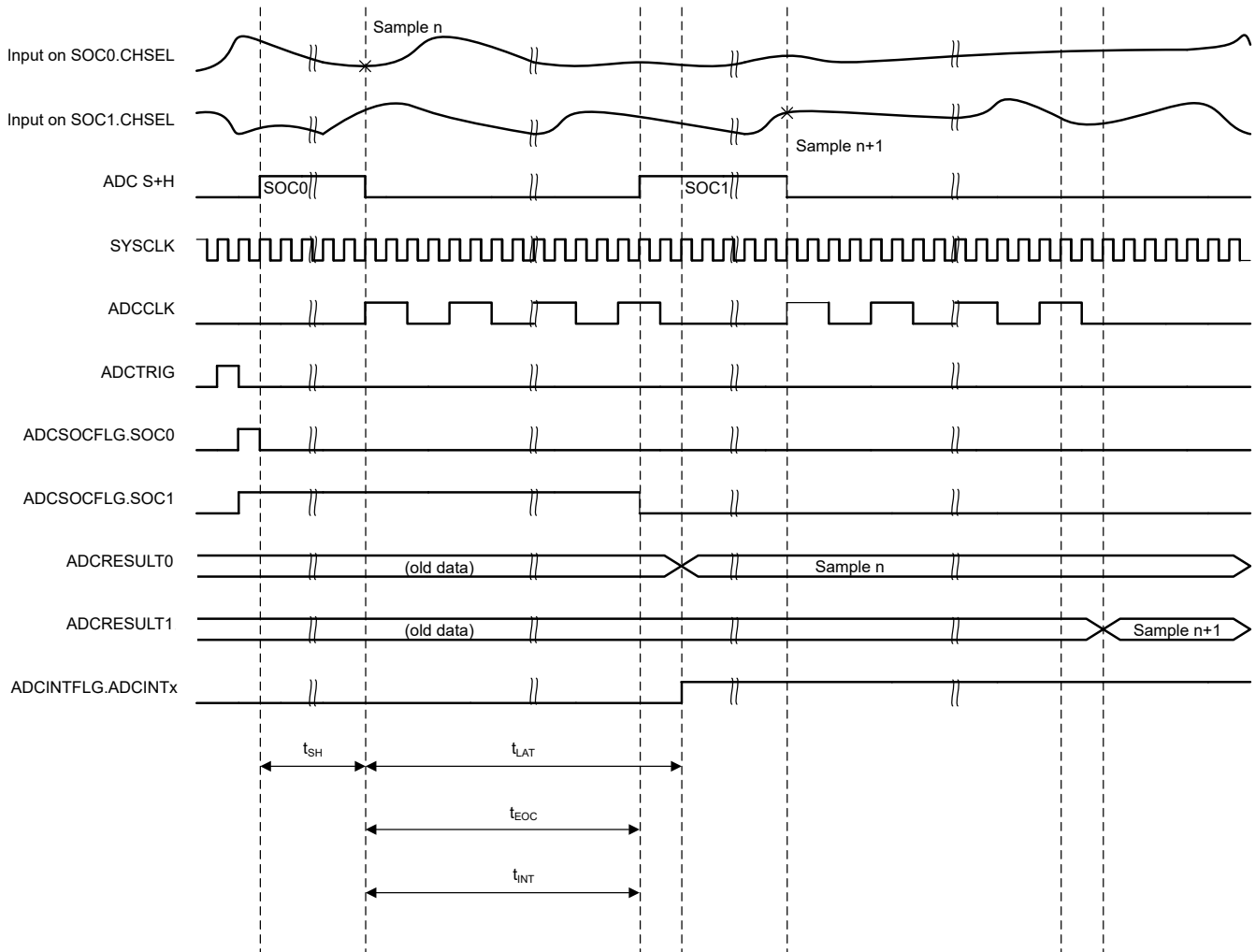
Figure 6-37. ADC Timings
