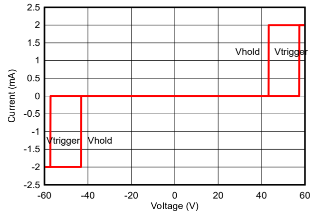
Figure 5-2. DC I-V Curve
