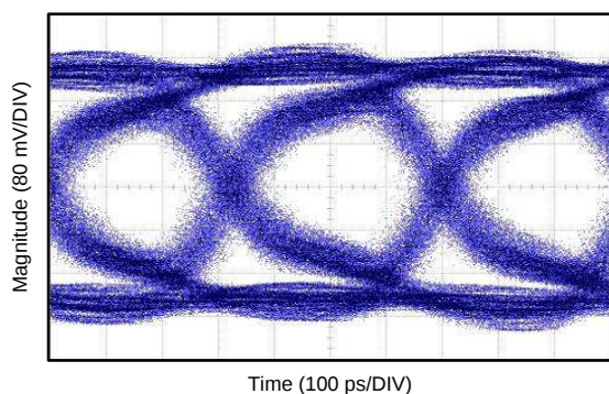
Figure 26. Serializer Eye Diagram at 2.73 Gbps Serial Data Rate
