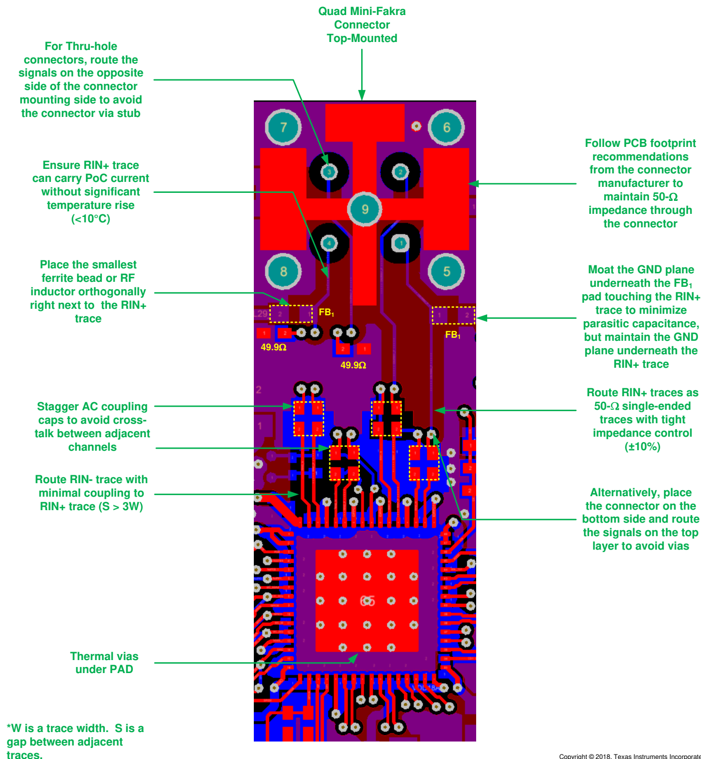
Figure 8-21. DS90UB960-Q1 Example PCB Layout With Quad Mini-Fakra Connector
