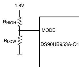
Figure 6-7. MODE Configuration
