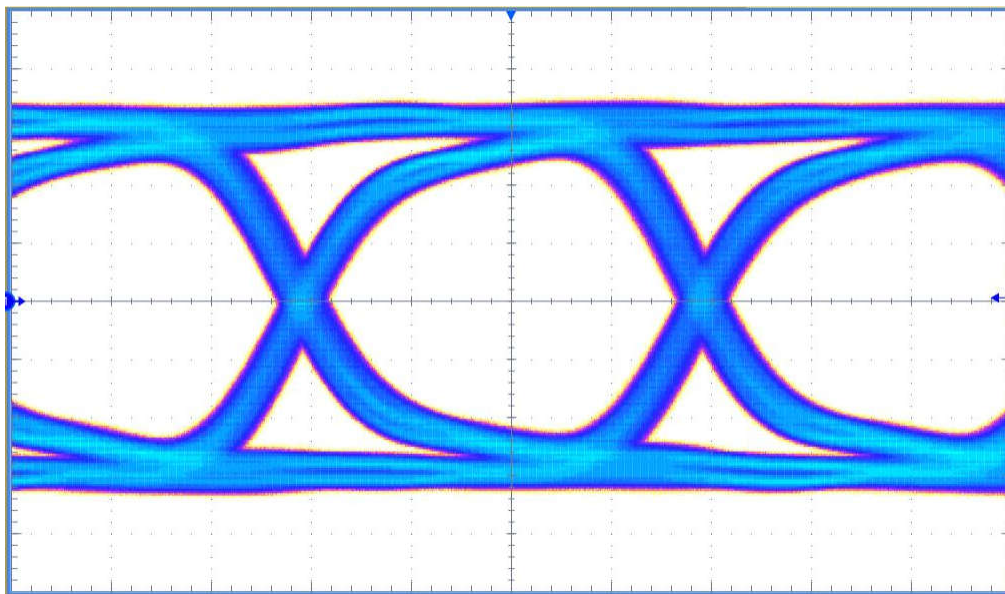
Figure 5-3. Eye Diagram at 4Gbps FPD-Link III Forward Channel Rate From Serializer Output Vertical Scale: 100mV/DIV Horizontal Scale: 62.5ps/DIV
