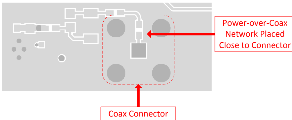
Figure 7-12. Power-over-Coax Layout
