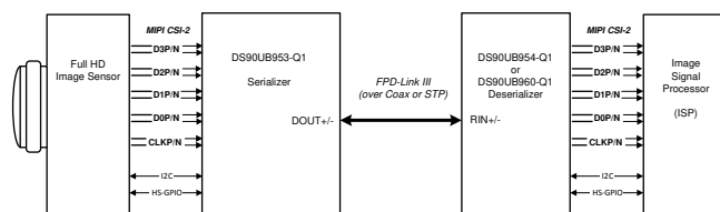
Typical Application
