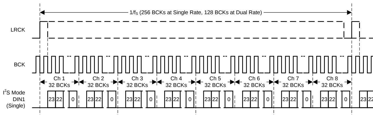
Figure 19. TDM Format
