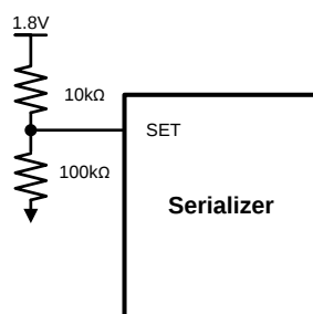
Figure 15. SET Pin configuration on DS90UA101-Q1
