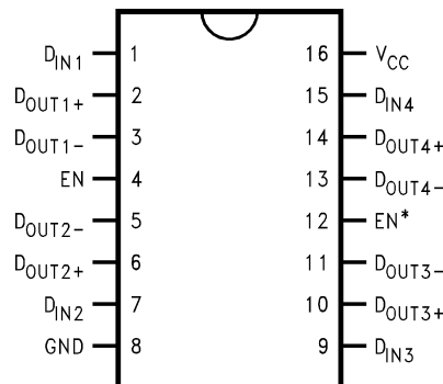
Figure 1. Dual-In-Line See Package Number NAC0016A or NAD0016A
