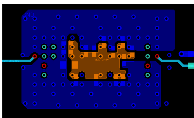
Figure 38. Microstrip Example, Bottom Layer
