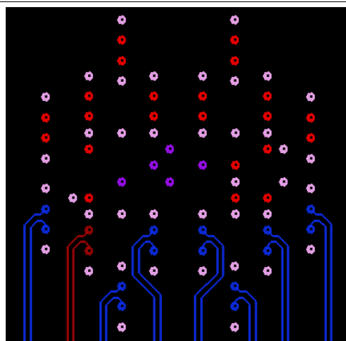
Figure 32. Stripline Example, Internal Signal Layer 1
