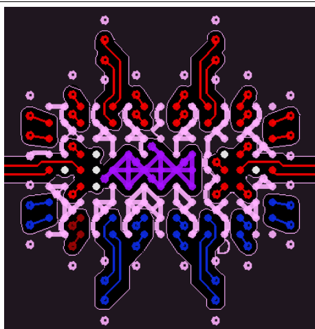
Figure 31. Stripline Example, Top Layer
