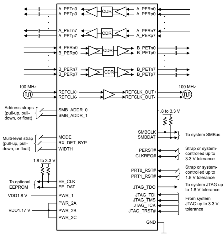
Simplified Schematic
