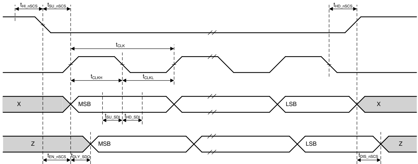
Figure 1. SPI Timing
