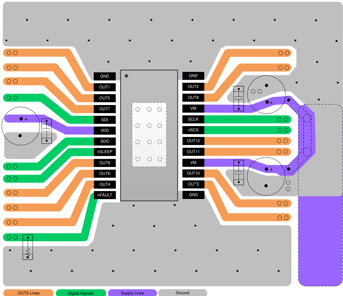
Figure 163. Layout Example
