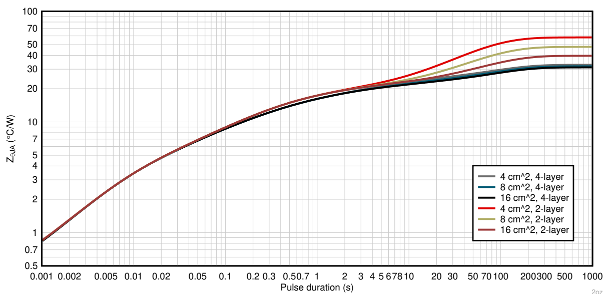
Figure 8-8. HTSSOP package Junction-to-ambient thermal impedance for 2-oz copper layouts
