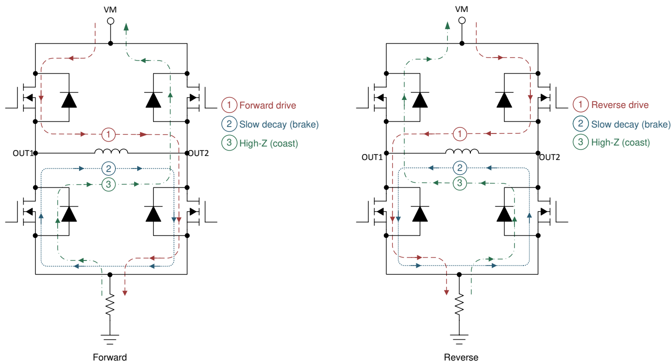
Figure 7-1. H-Bridge States
