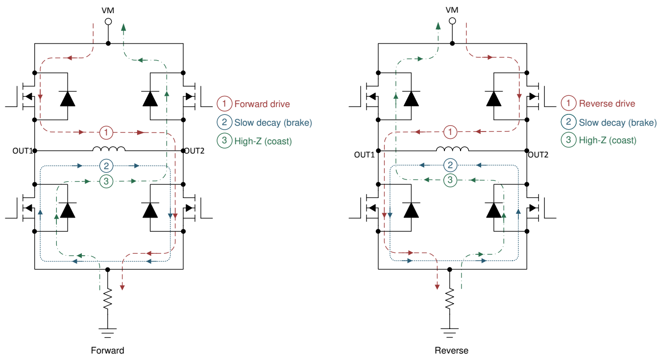
Figure 7-1. H-Bridge States
