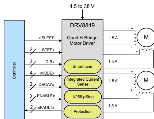
Simplified Schematic
