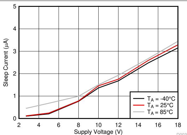
Figure 6-5. Sleep Mode Supply Current ( I_{VMQ} ) vs Supply Voltage ( V_{VM} )
