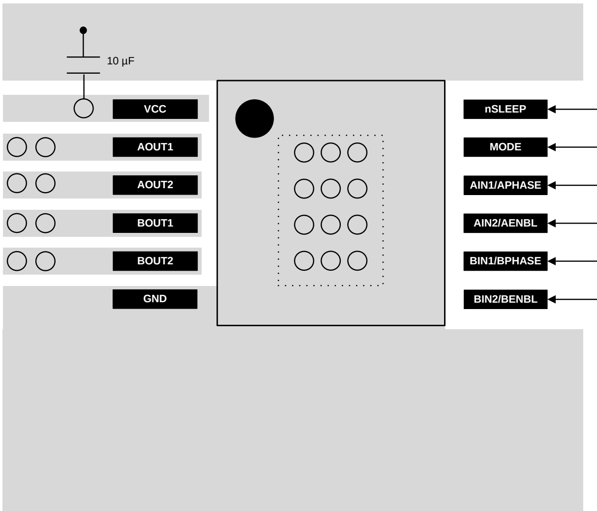
Figure 8. Layout Recommendation
