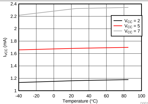
Figure 3. V CC Operating Current, fPWM = 50 kHz, No Load
