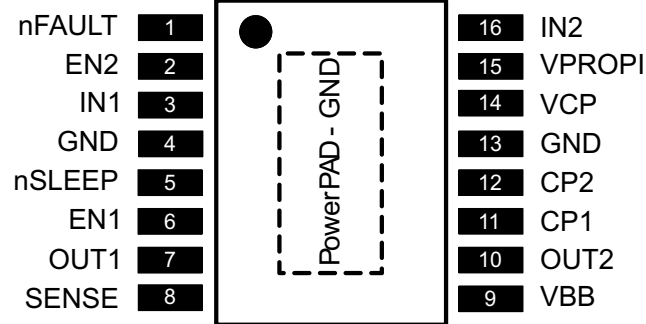
Pin Functions
