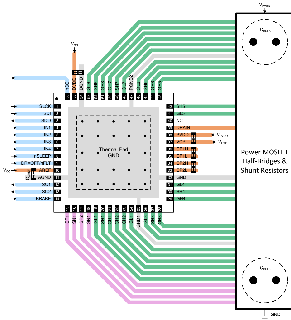
Figure 9-9. Layout Example
