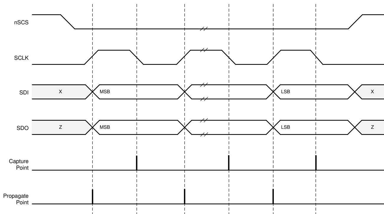
Figure 7-54. SPI Transaction
