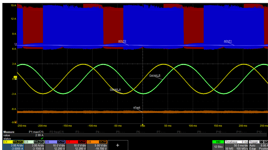
Figure 8-5. 1/256 microstepping at 6400 pps with I_{FS} = 3 A
