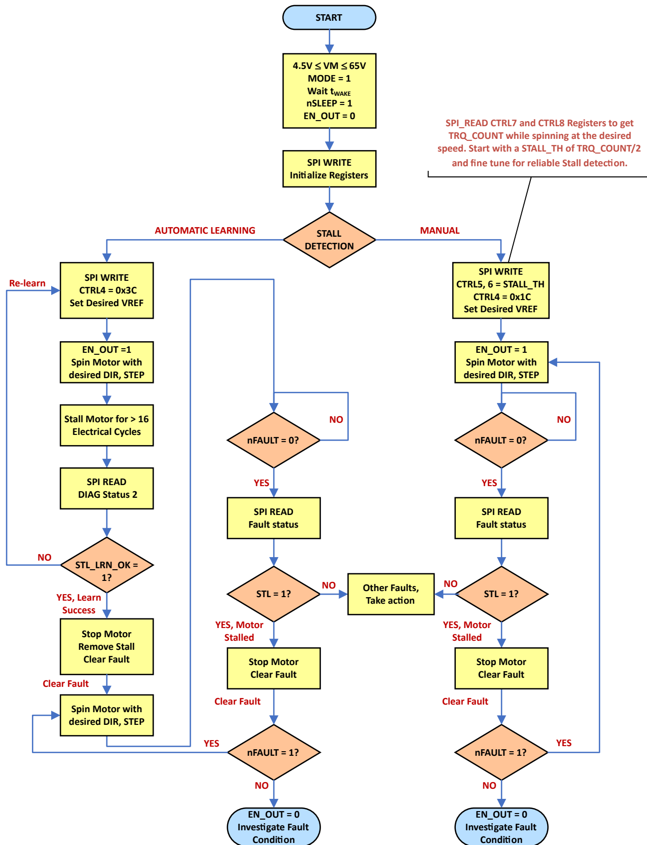
Figure 7-43. Stall learning flowchart
