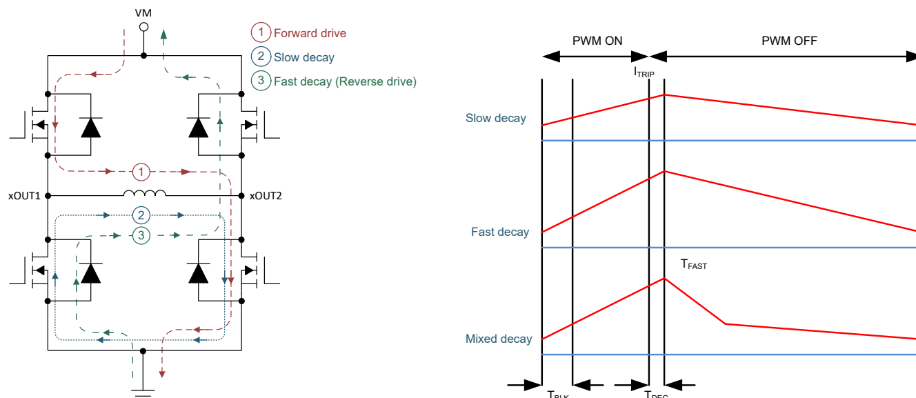
Figure 7-12. Decay Modes
