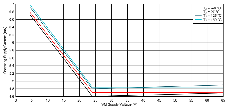
Figure 6-4. Operating supply current, VCC = External 5 V
