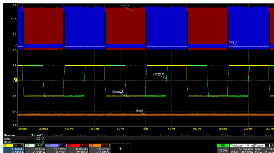
Figure 8-3. Full-step at 25 pps with I_{FS} = 3 A
