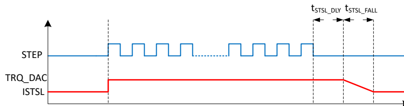
Figure 7-11. Standstill Power Saving Mode
