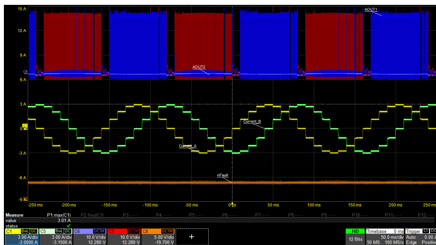
Figure 8-4. 1/4 microstepping at 100 pps with I_{FS} = 3 A
