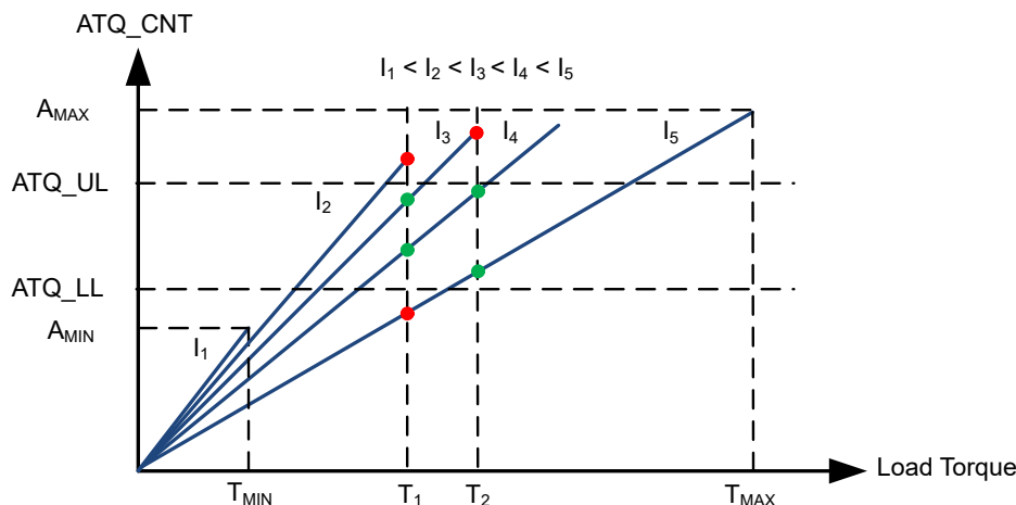
Figure 7-27. ATQ_CNT as a function of load torque
