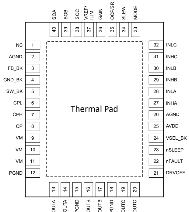
Figure 6-2. DRV8316CT-Q1 40-Pin VQFN With Exposed Thermal Pad Top View
