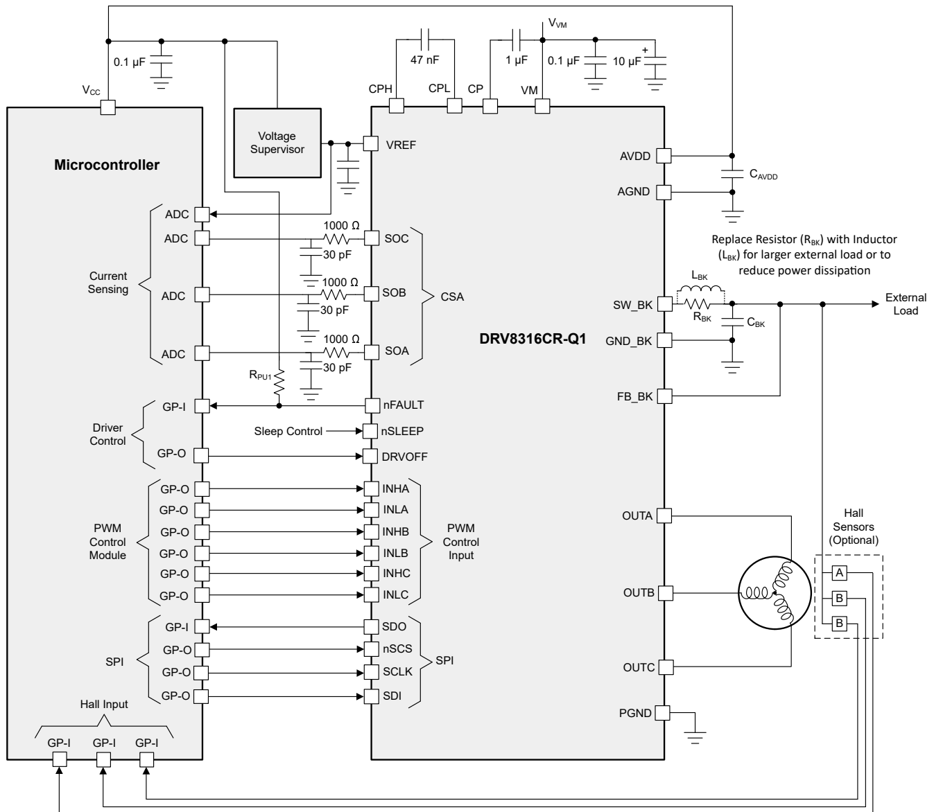
Figure 9-1. Primary Application Schematic
