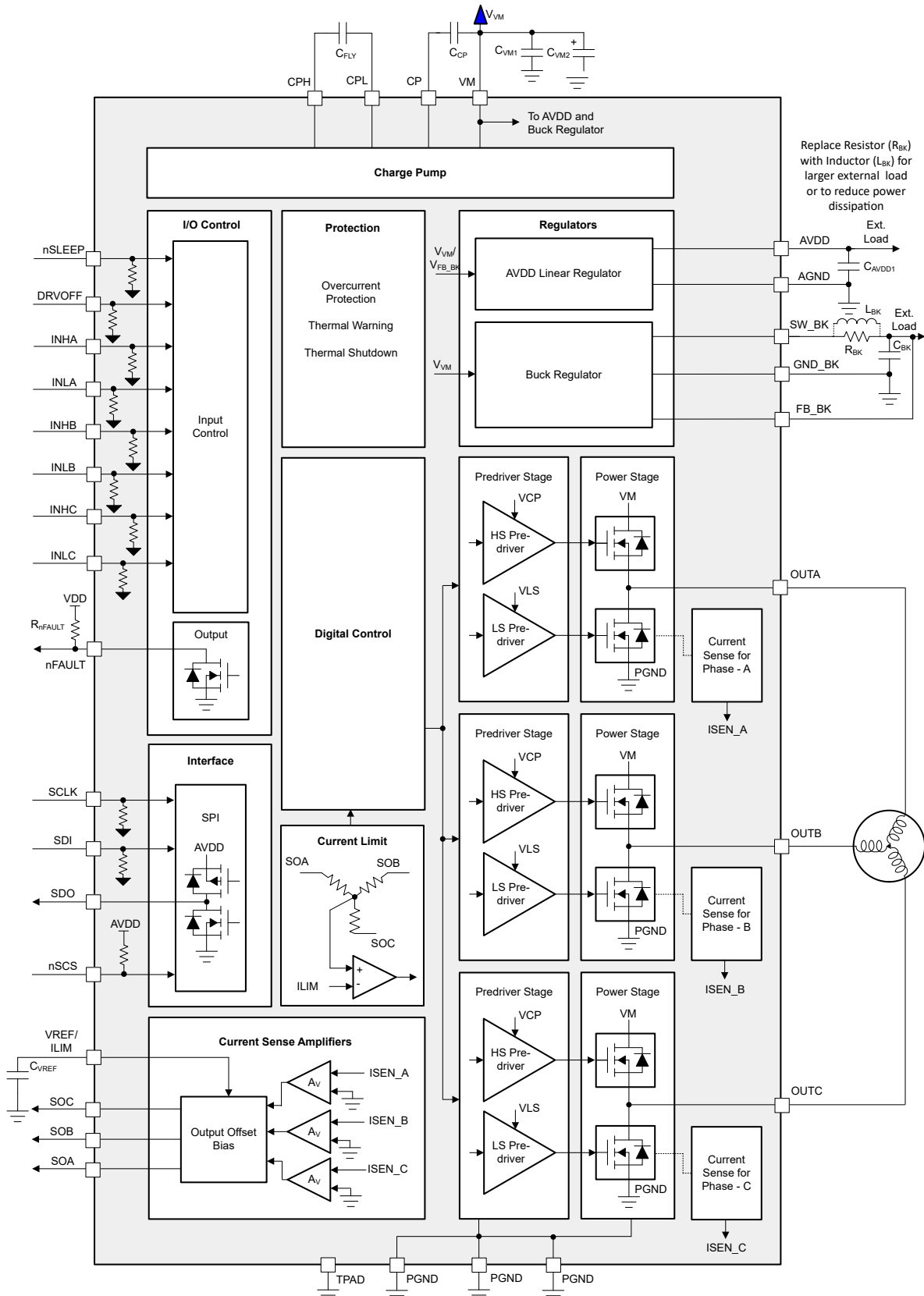
Figure 8-1. DRV8316CR-Q1 Block Diagram
