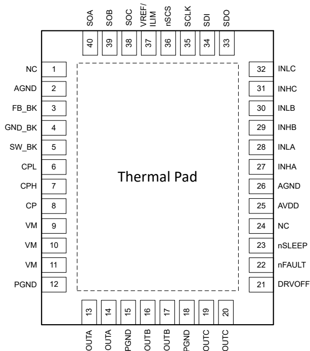
Figure 6-1. DRV8316CR-Q1 40-Pin VQFN With Exposed Thermal Pad Top View
