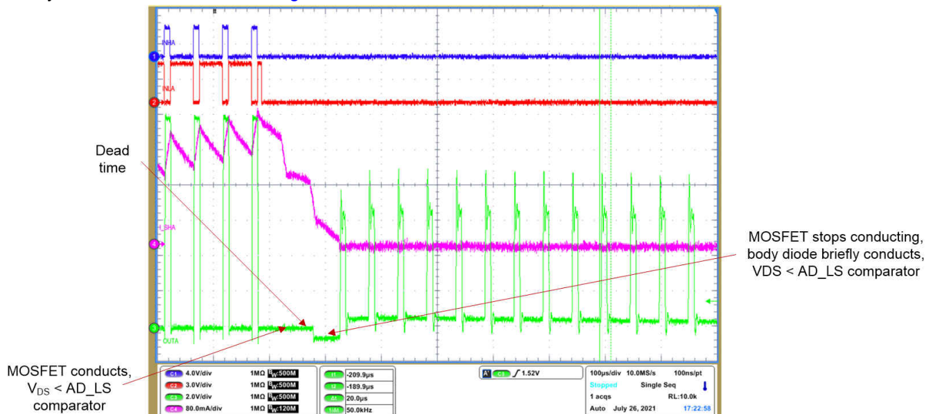
Figure 9-3. Active demagnetization enabled in DRV8316C-Q1
