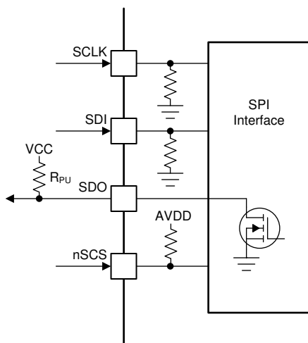
Figure 8-7. DRV8316CR-Q1 SPI Interface
