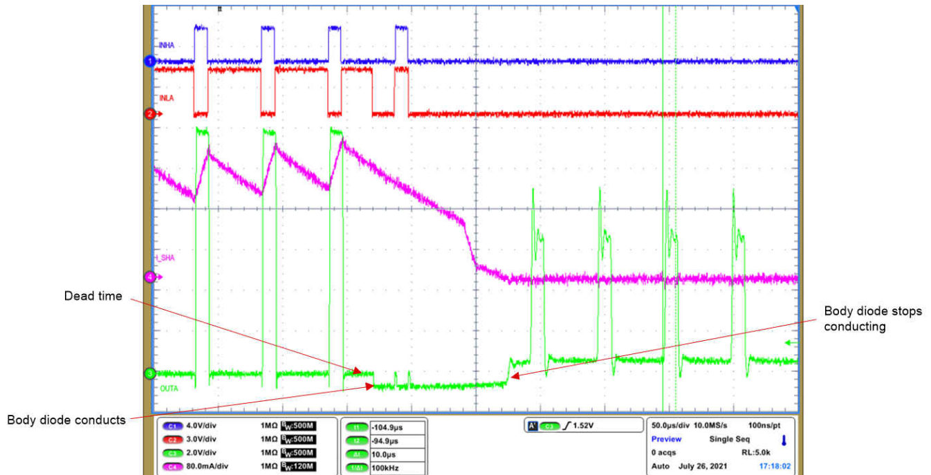
Figure 9-2. Active demagnetization disabled in DRV8316C-Q1
