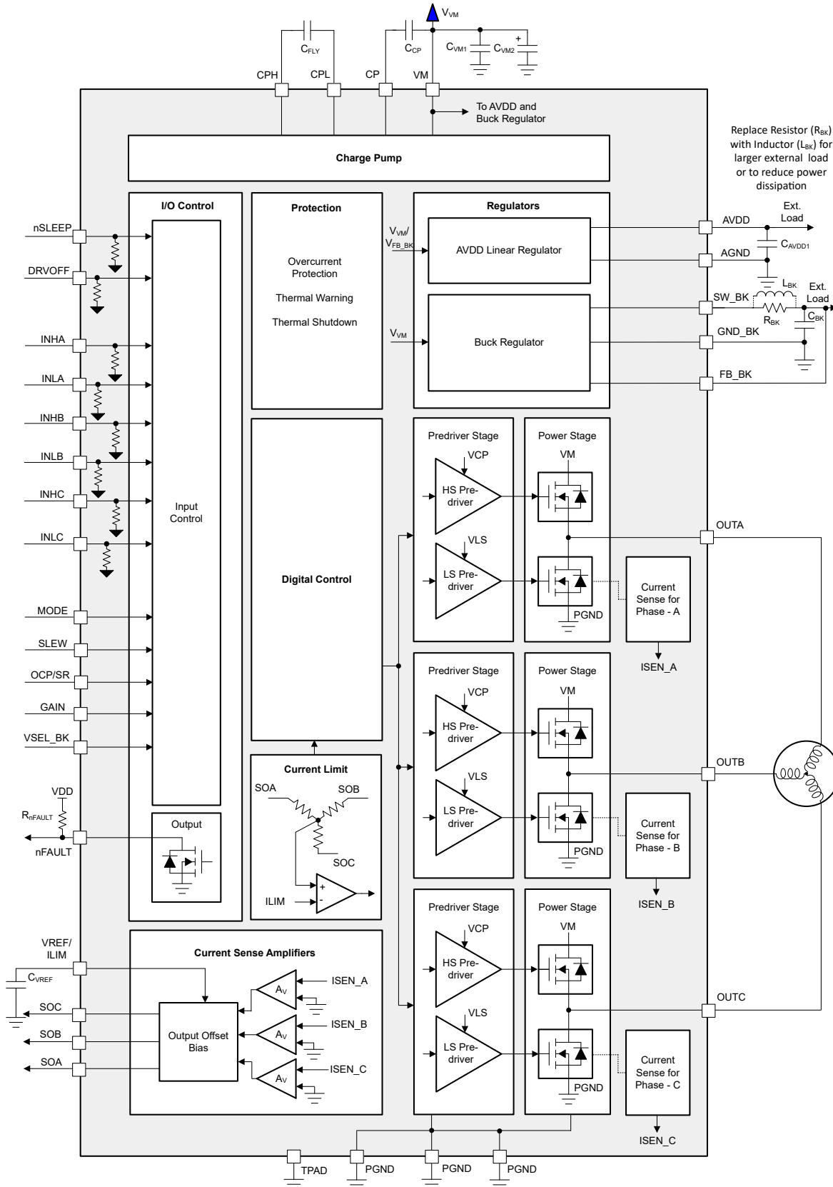
Figure 8-2. DRV8316CT-Q1 Block Diagram
