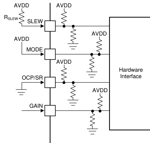
Figure 8-8. DRV8316CT-Q1 Hardware Interface
