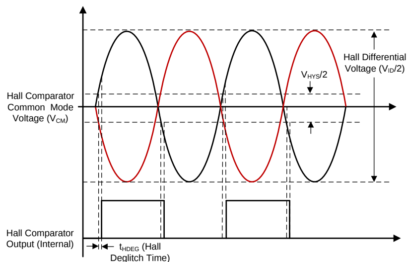
Figure 20. Hall Comparators
