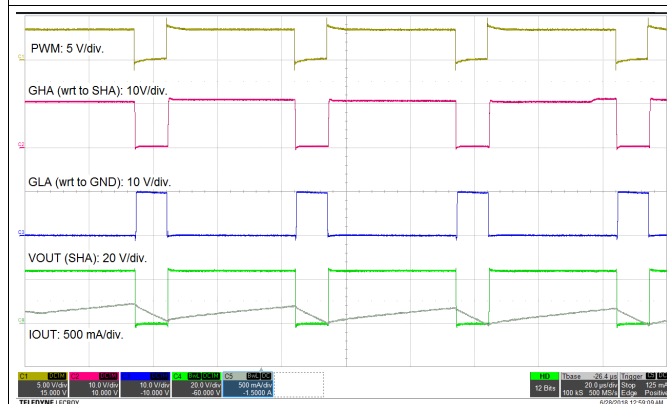
Figure 33. Gate Drive 80% Duty Cycle
