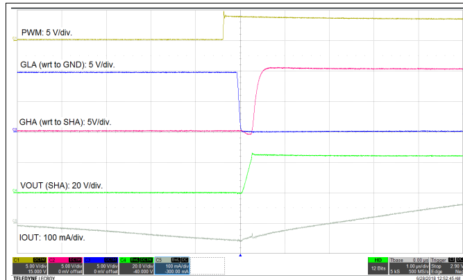
Figure 31. IDrive Maximum Setting
