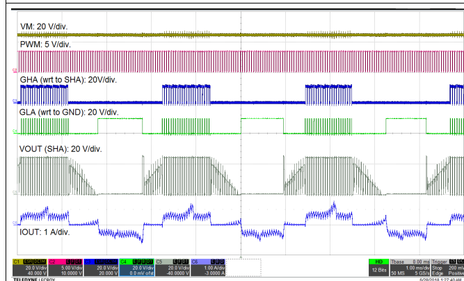
Figure 35. Motor Operation at 80% PWM Duty
