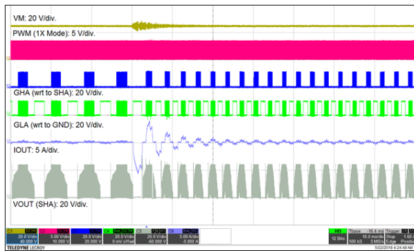
Figure 53. Motor Starting With PWM Duty Change
