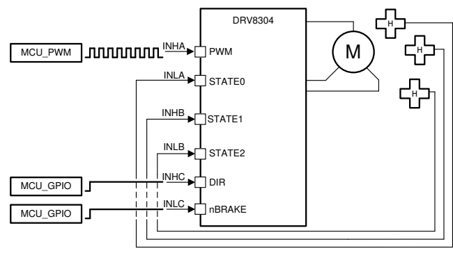
Figure 13. 1x PWM—Hall Sensor
