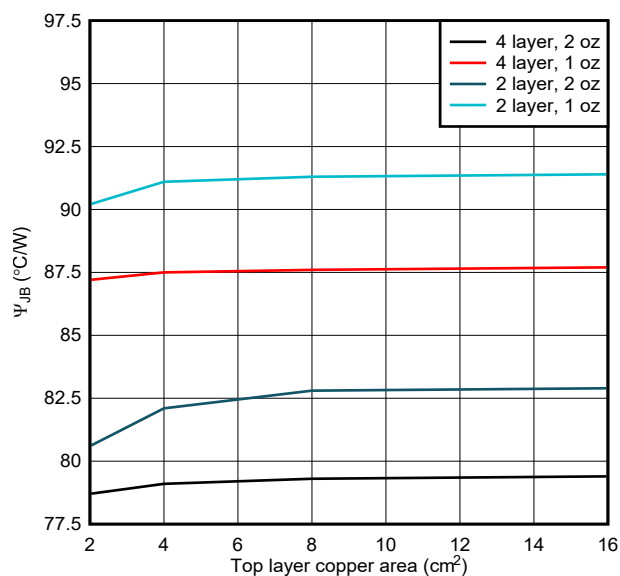
Figure 9-31. SOT, junction-to-board characterization parameter vs copper area
