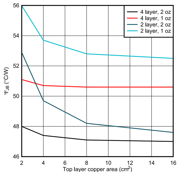
Figure 9-29. WSON, junction-to-board characterization parameter vs copper area
