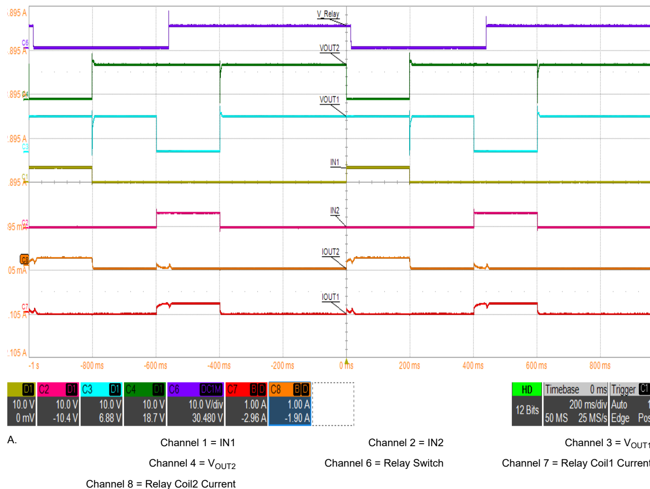
Figure 9-22. PWM driving for dual-coil relay
