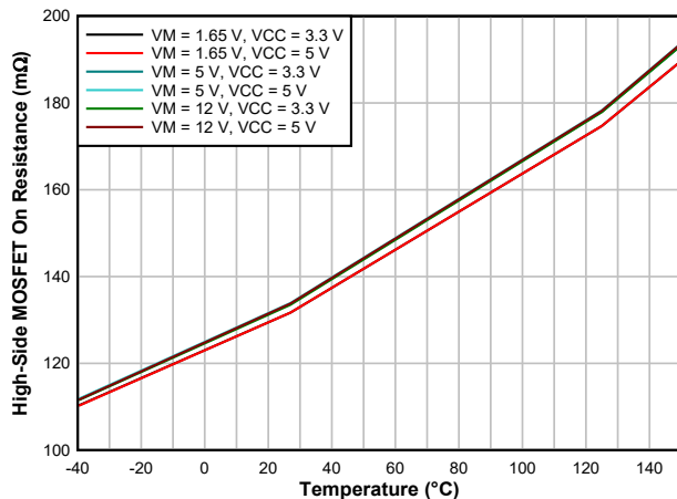
Figure 7-3. High-Side MOSFET On Resistance (mΩ)
