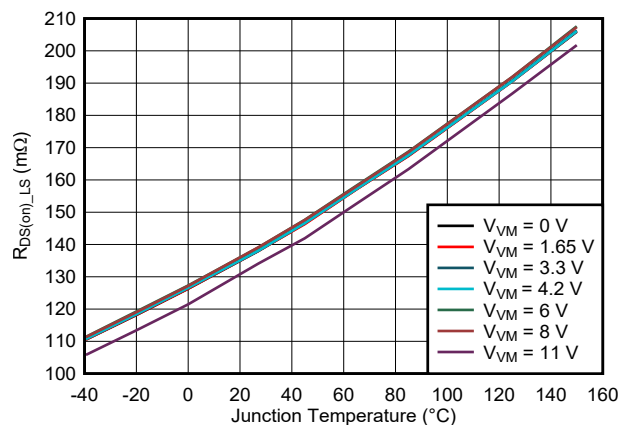
Figure 7-12. Low-Side R_{DS(on)} vs. Junction Temperature ( T_J )
