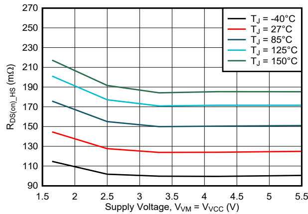
Figure 7-11. High-Side R_{DS(on)} vs. Supply Voltage
