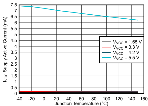
Figure 7-8. Active Current ( I_{VCC} ) vs. Junction Temperature ( T_J )
