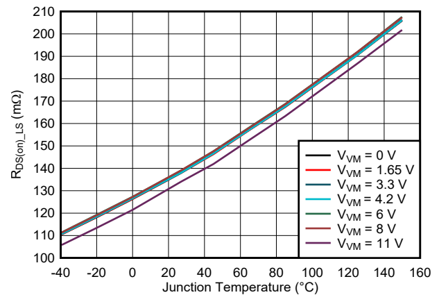
Figure 7-14. Low-Side R_{DS(on)} vs. Junction Temperature ( T_J )
