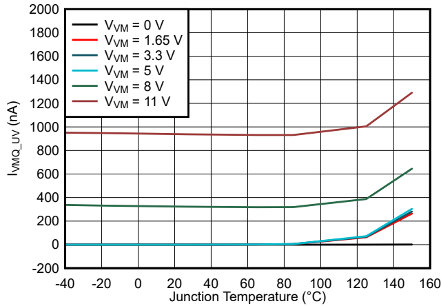
Figure 7-9. VM supply current when VCC is low ( I_{VMQ\_UV} ) vs. Junction Temperature ( T_J )
