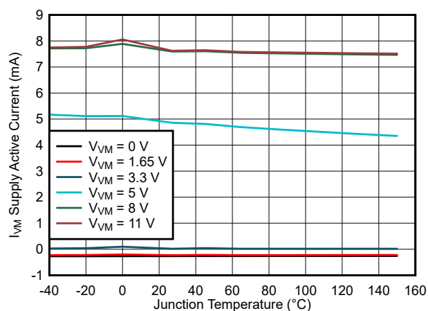
Figure 7-6. Active Current ( I_{VM} ) vs. Junction Temperature ( T_J )
