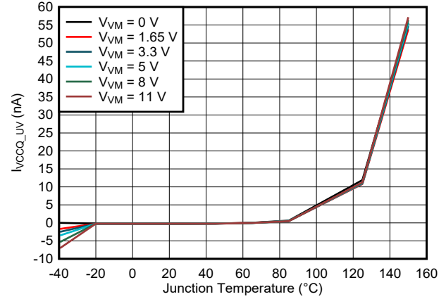
Figure 7-10. VCC supply current when VCC is low ( I_{VCCQ\_UV} ) vs. Junction Temperature ( T_J )
