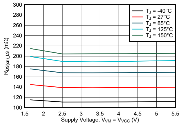
Figure 7-13. Low-Side R_{DS(on)} vs. Supply Voltage
