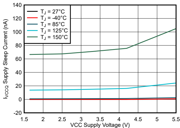
Figure 7-3. Sleep Current ( I_{VCCQ} ) vs. Supply Voltage ( V_{VCC} )
