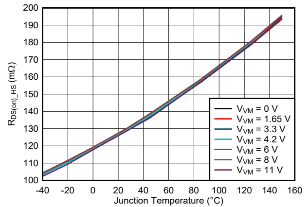
Figure 7-12. High-Side R_{DS(on)} vs. Junction Temperature ( T_J )
