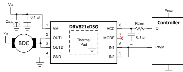
Figure 9-11. Half-bridge mode used as a low-side driver with outputs paralleled
