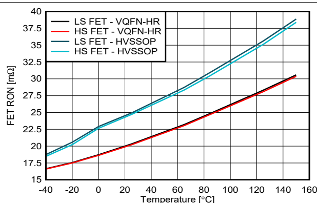
Figure 6-11. R_{HS\_ON} & R_{LS\_ON} vs Temperature at V_{VM} = 13.5 V
