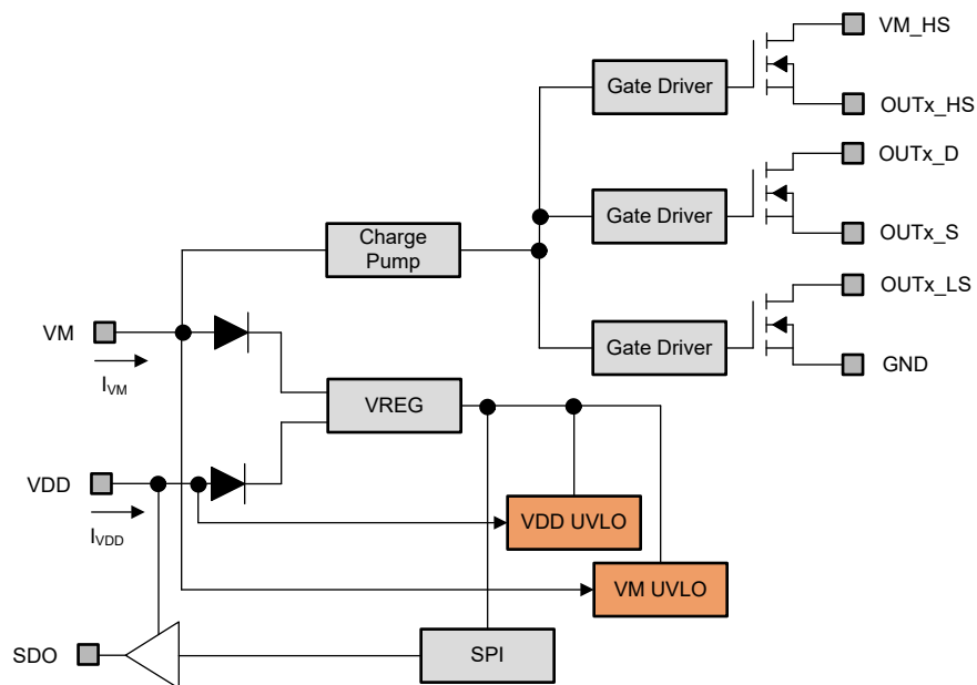
Figure 7-3. Internal Power Supply Architecture
