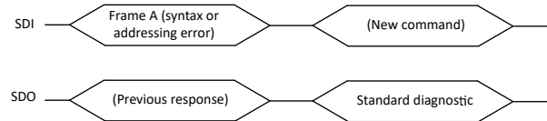
Figure 7-31. Response After a Command Syntax Error
