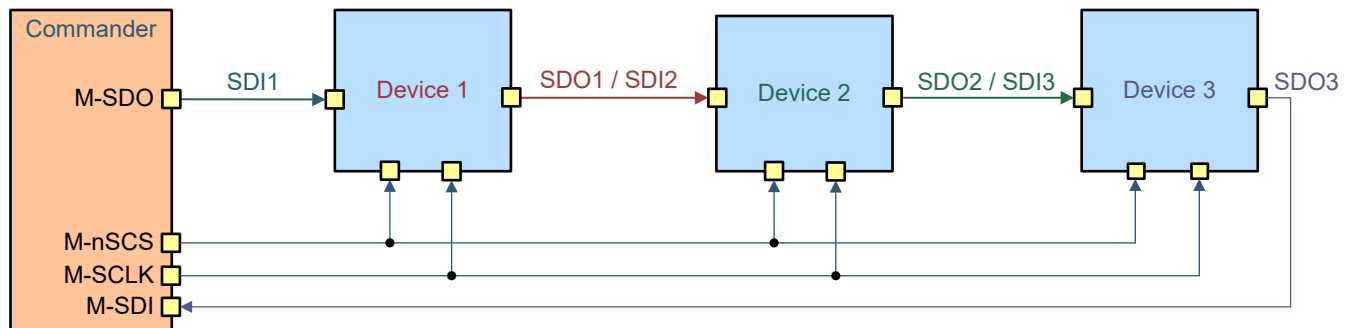
Figure 7-26. Daisy Chain Configuration
