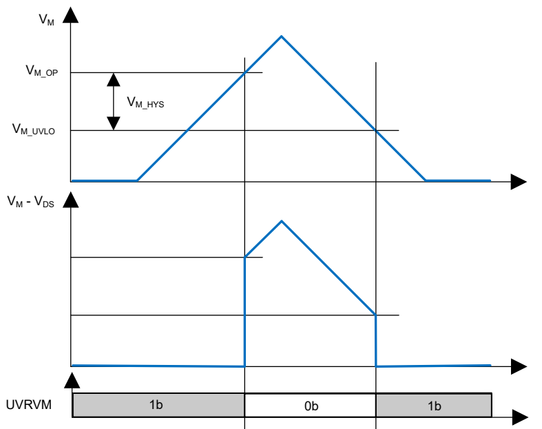
Figure 7-13. V_M Undervoltage Behavior
