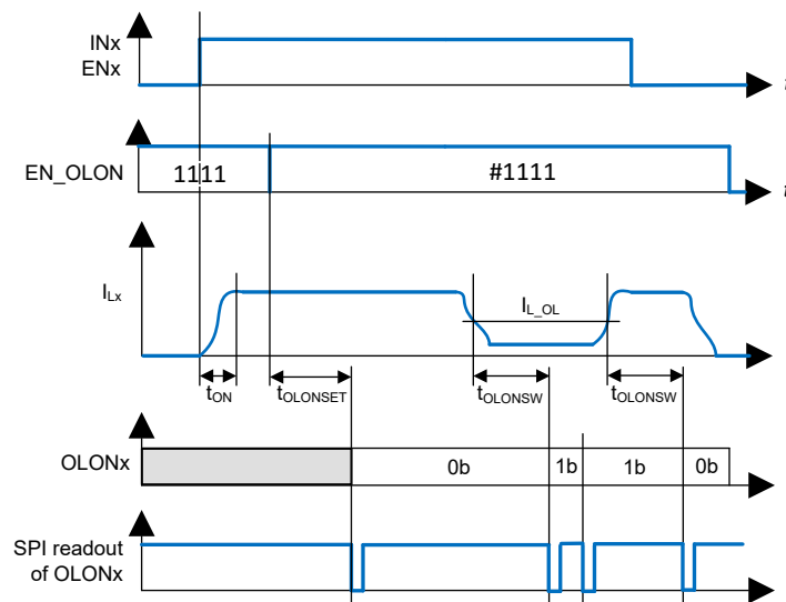
Figure 7-22. Open Load at ON Timings (direct Channels Diagnosis)
