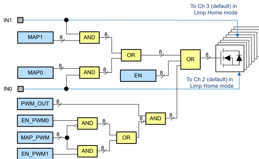
Figure 7-12. PWM Generator Mapping
