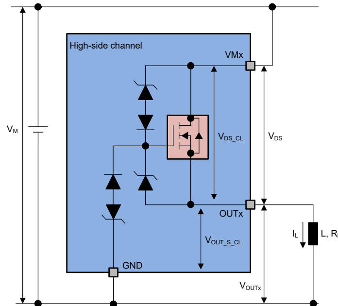
Figure 7-10. Output Clamp for high-side channel
