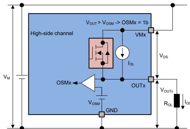
Figure 7-21. Output Status Monitor - High-side Channels
