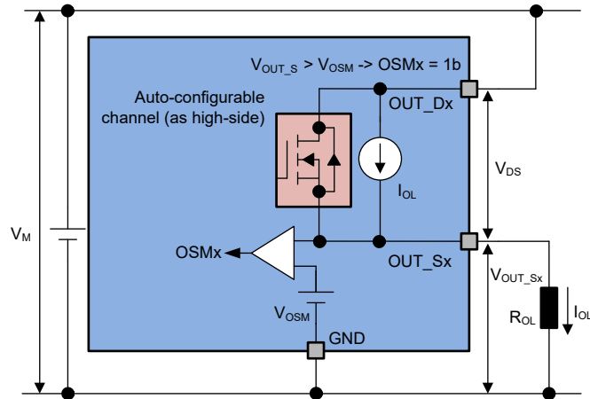
Figure 7-19. Output Status Monitor - Auto-configurable Channel as High-side
