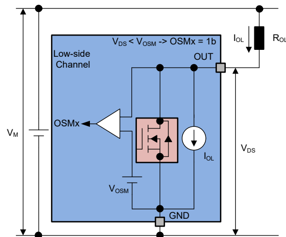
Figure 7-18. Output Status Monitor - Low-side Channels
