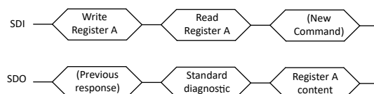
Figure 7-28. Register content sent back to microcontroller
