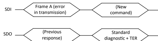
Figure 7-29. Response After a Error in Transmission
