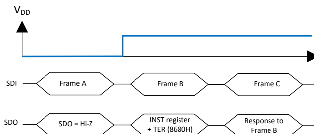
Figure 7-30. Response After Coming Out Of Power-On Reset at V_{DD}
