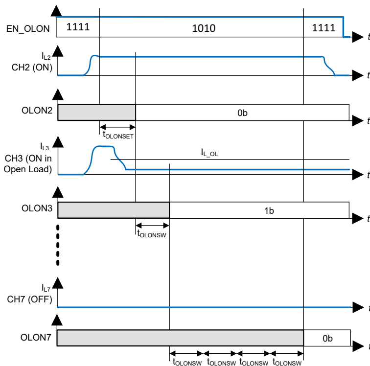
Figure 7-23. Open Load at ON Timings (Diagnosis Loop - Channels Driven by Micro-controller)
