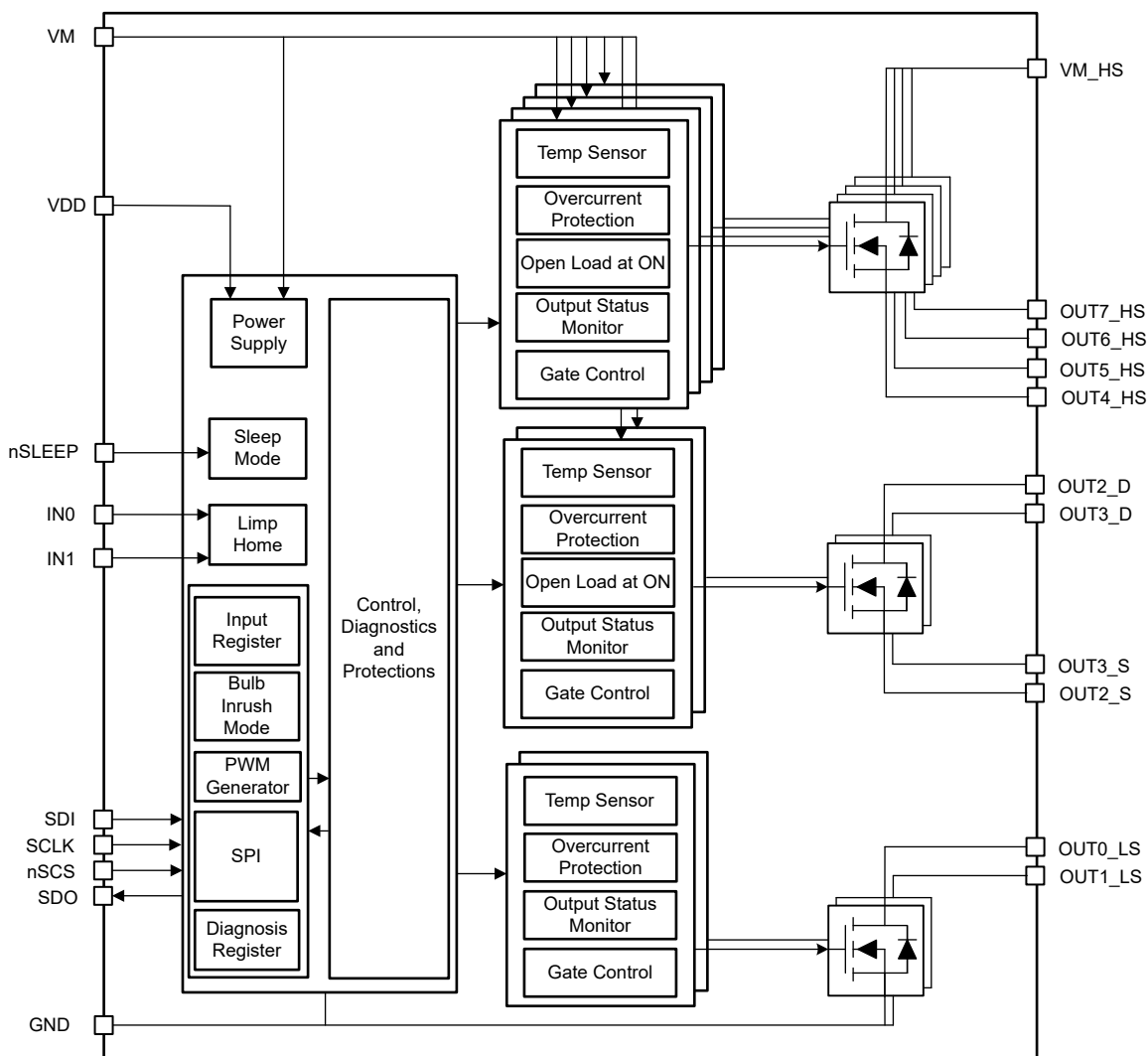
Figure 7-1. DRV81242-Q1 Functional Block Diagram
