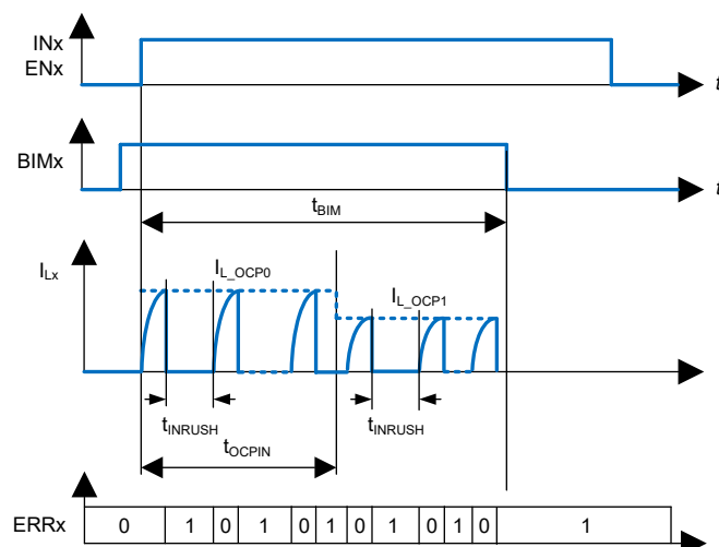
Figure 7-11. Bulb Inrush Mode (BIM) Operation
