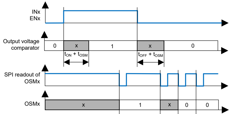
Figure 7-17. Output Status Monitor timing
