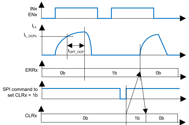
Figure 7-15. Latch OFF at Overcurrent
