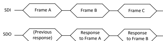
Figure 7-27. Relationship Between SDI and SDO During SPI Communication
