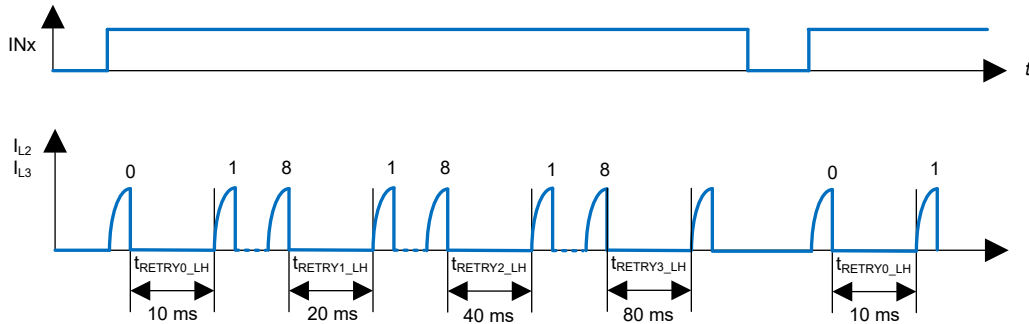
Figure 7-16. Restart Timer in Limp Home
