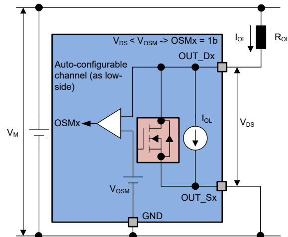
Figure 7-20. Output Status Monitor - Auto-configurable Channel as Low-side
