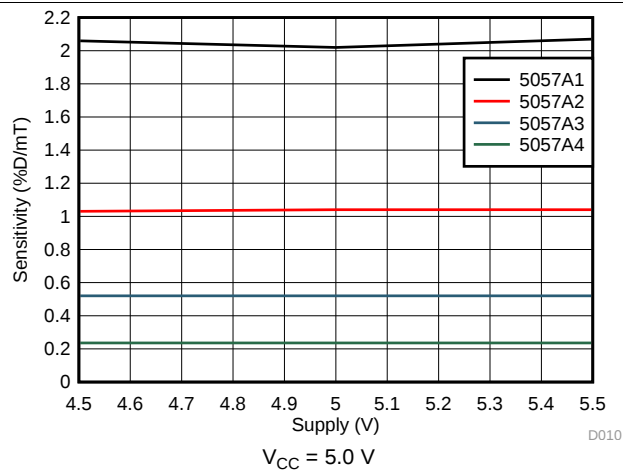
Figure 1. Sensitivity vs Supply Voltage
