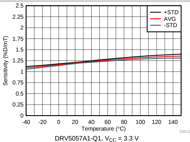
Figure 5. Sensitivity vs Temperature
