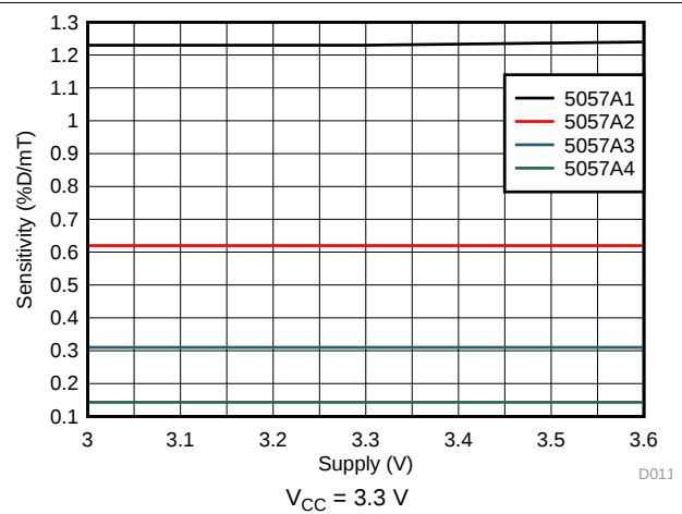
Figure 2. Sensitivity vs Supply Voltage
