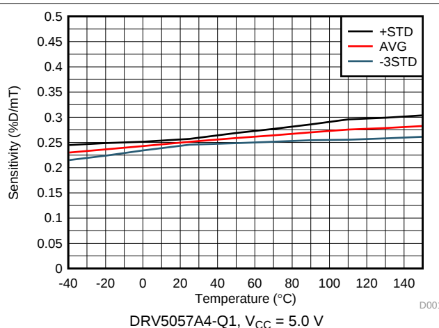
Figure 10. Sensitivity vs Temperature
