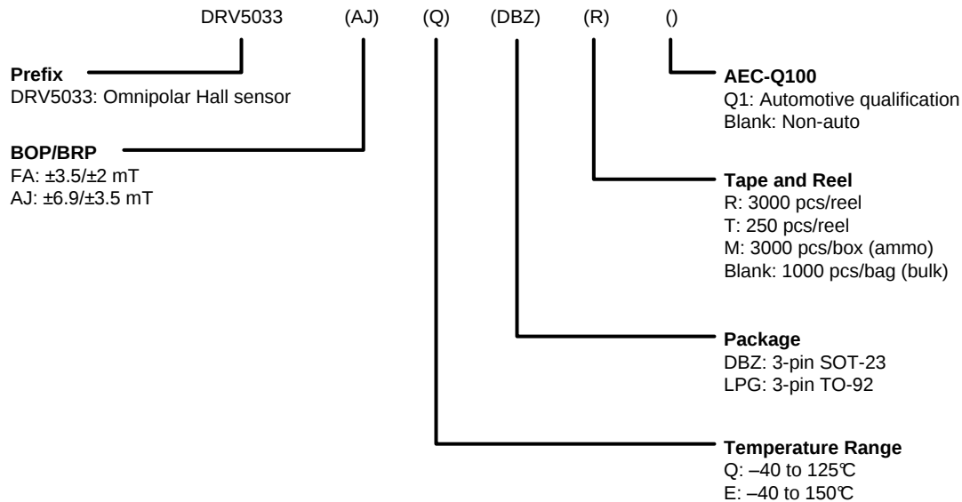
Figure 24. Device Nomenclature
