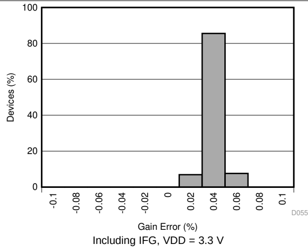
Figure 31. Shunt-Sense Amplifier Gain Error Histogram
