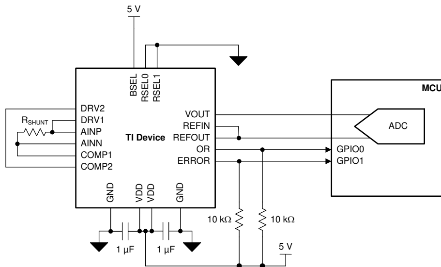
Figure 67. Linear-Position Sensing
