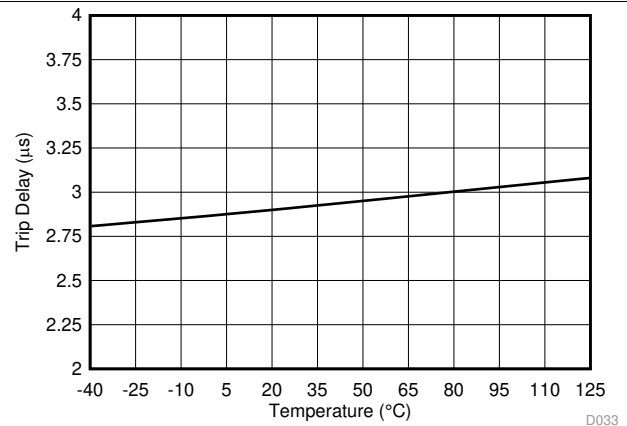
Figure 38. \overline{\text{OR}} Pin Trip Delay vs Temperature
